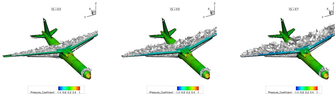
Figure 12 - Wave drag sources based on Euler simulations on the reference Strut-Braced Wing configuration
