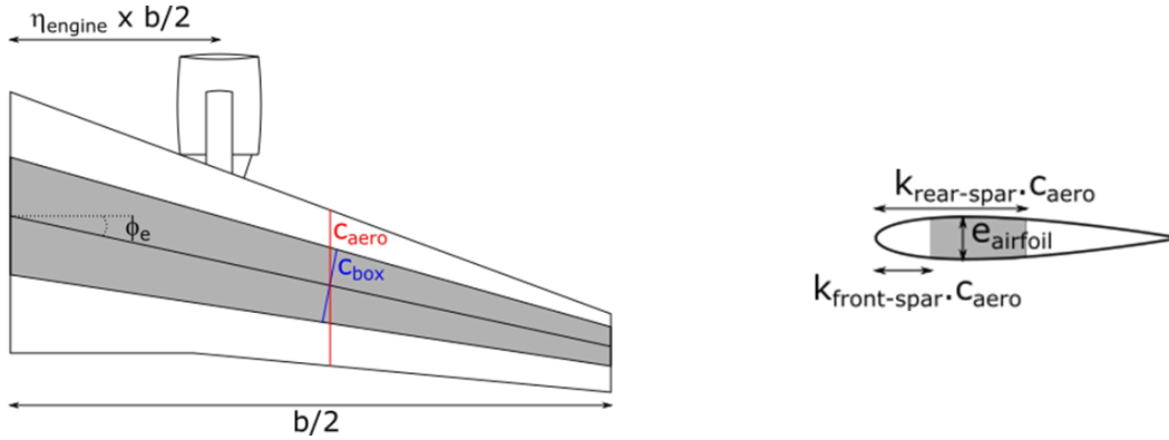
Figure 20 - Wingbox parametrization for loads computation
