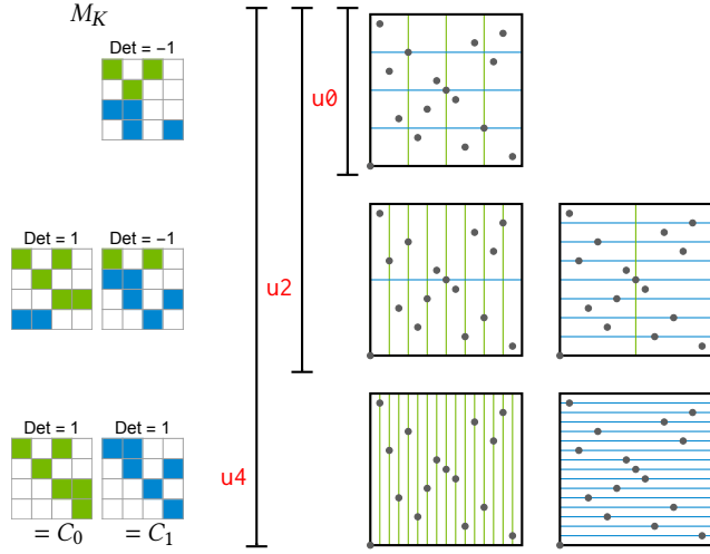
Fig. 3. Modifiers u_{m'} illustrated for the relaxed (0, m, s) -net constraint in 2 dimensions, base 2, and for 2^4 samples: u_0 corresponds to a stratification test enforcing one sample per (\frac{1}{4} \times \frac{1}{4}) strata, u_4 amounts to a complete (0, m, 2) -net check, and u_2 leads to intermediate constraints. Such properties can be assessed by checking the determinant of the M_K matrices: 2 rows from C_0 and C_1 ( u_0 ), 1 row from C_0 , three from C_1 and conversely ( u_2 ), or the full C_0 and C_1 matrices ( u_4 ). The strata depicted in the unit squares on the right are the elementary intervals underlying the displayed (0, 4, 2) -net.
