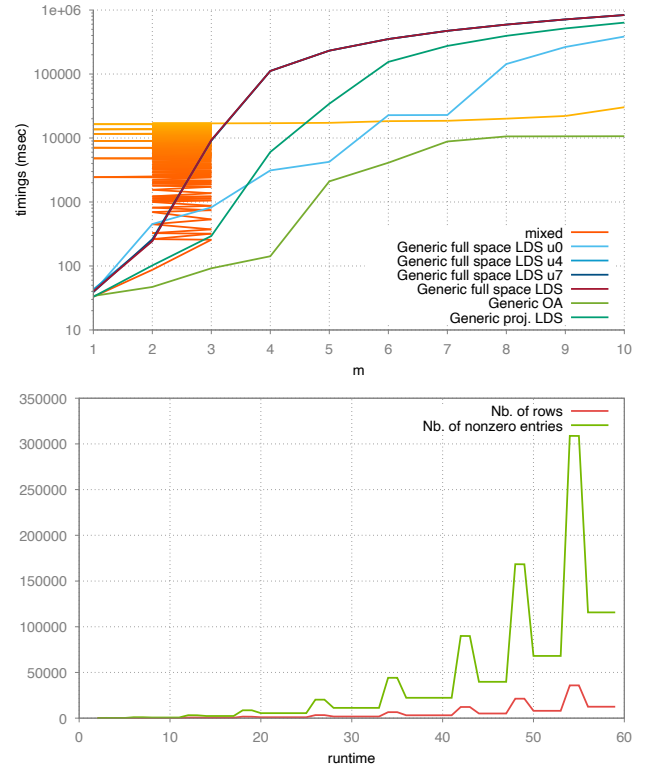
Fig. 5. Performance: On the top we show the timings of the MatBuilder solver as a function of the matrix size m . For the mixed profile, the plots show several backtracks for small m before being able to expand the matrices ( u4 and u7 have the same timings). At the bottom, the size of the reduced integer linear programs are shown during execution (number of rows and number of nonzero entries) for the generic-full-space-LDS profile (most difficult one in our tests). For this profile, up to 60 calls to the internal integer linear program simplification procedure have been performed.
