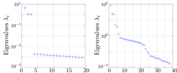
FIGURE 5. Eigenvalues \lambda_i for the weakly (left) and strongly (right) coupled cases using 500 samples.
