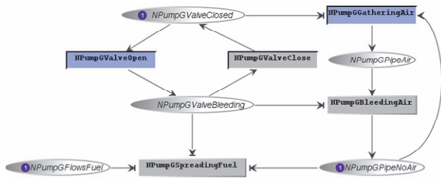
Figure 2. North Pump-G Valve Including Erroneous Events The example shows the modeling of erroneous human-system interaction behavior (bleeding pipes while pumps in operation) and of a system-related erroneous event (pipes gathering air).
