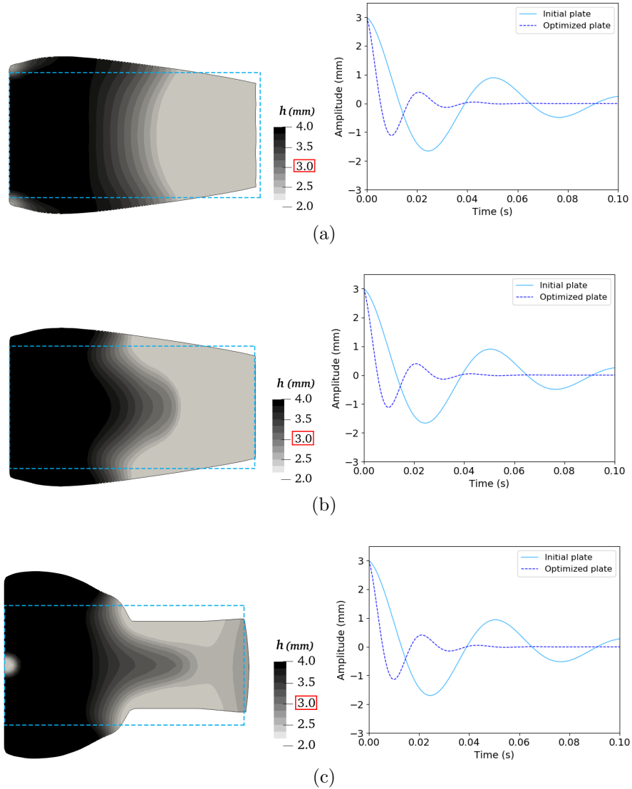
FIGURE 17. Thickness profiles and free vibration amplitudes of the considered plates for a Zener material and different Poisson's ratios (a) \nu_1 = 0.498 (b) \nu_1 = 0.48 (c) \nu_1 = 0.4 .
