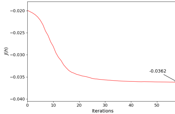
FIGURE 13. Cost function convergence with respect to the number of iterations of the shape optimization for the generalized Maxwell material.
