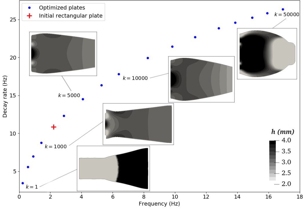
FIGURE 20. Decay rate with respect to the vibration frequency and design representations for plate inverse damping \mathcal{J}(h, \Omega) = \omega_i(h, \Omega) + k \frac{1}{\omega_r(h, \Omega)} optimization.
