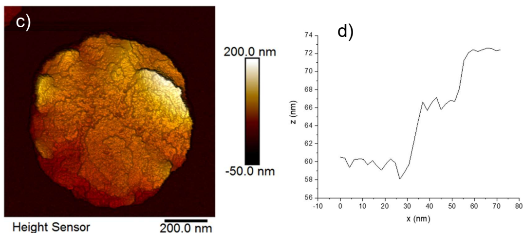
Figure 7. liquid AFM just after deposition on a functionalized substrate of the “just prepared” pre-heated mixture (reaction mixture with \text{FeSt}_2 ) a) and after ageing b). High magnification of “aged” nanostructures c) and AFM profile of an “aged” nanostructure d) from figure c).
