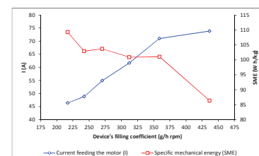
Fig. 3. Current feeding the motor and specific mechanical energy as a function of the device's filling coefficient.
