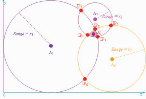
Fig.1 Finding Intersection Points (IPs)
