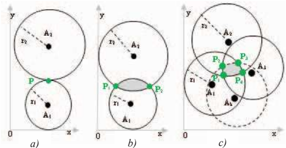
Fig. 3 SCOP as one, two, k TIPs
