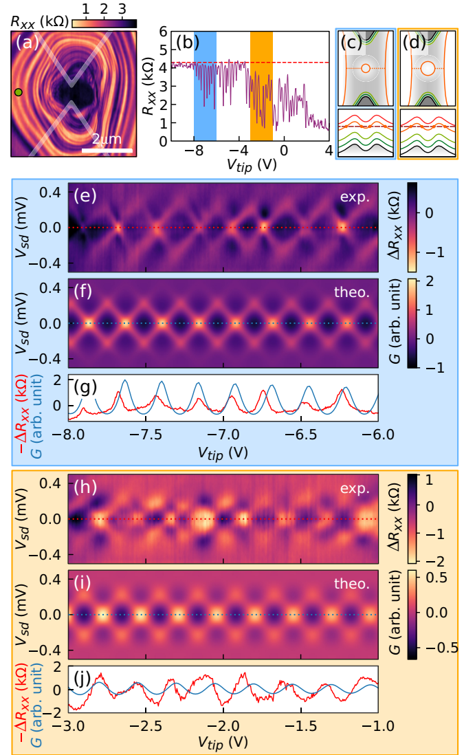
FIG. 2. (a) SGM map obtained by recording R_{xx} as a function of the tip position at B = 7.3 \text{ T} [blue dashed line in Fig. 1(d)] and with V_{tip} = 0 \text{ V} (depleting tip due to the work function difference with the sample surface). The QPC borders are indicated by the white shaded area. (b) Evolution of R_{xx} with V_{tip} for the tip position indicated with a green dot in (a). The red dashed lines indicates the 4.3 \text{ k}\Omega plateau. (c), (d) Evolution of the QHECs spatial configuration with V_{tip} in the vicinity of the constriction (top panels) and the corresponding Landau level positions compared to the Fermi energy E_F (bottom panel). (c) and (d) correspond, respectively, to the blue and orange regions in (b). (e), (f) Experimental map of \Delta R_{xx} and simulated map of G , respectively, as a function of V_{sd} and V_{tip} [blue region in (b)]. The maps feature diamond patterns. (g) \Delta R_{xx} at V_{sd} = 0 from (e) in red and G versus V_{tip} from (f) in blue. (h), (i) Experimental map of \Delta R_{xx} and simulated map of G , respectively, as a function of V_{sd} and V_{tip} [orange region in (b)]. The maps feature checkerboard patterns. (j) \Delta R_{xx} at V_{sd} = 0 from (h) in red and G versus V_{tip} from (i) in blue.
