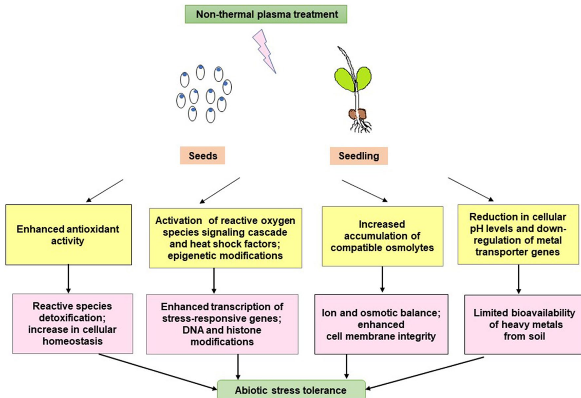
Fig. 4 Plausible non-thermal plasma elicited responses in plants against various abiotic stresses. Pre-treatment of seeds or seedlings with non-thermal plasma could i induce synthesis of antioxidants that scavenge excess reactive species and re-establish homeostasis, ii activate several transcription factors that trigger the expression of stress-responsive genes and epigenetic changes lead to DNA and histone protein modifications, iii accumulation of soluble osmolytes helps to
