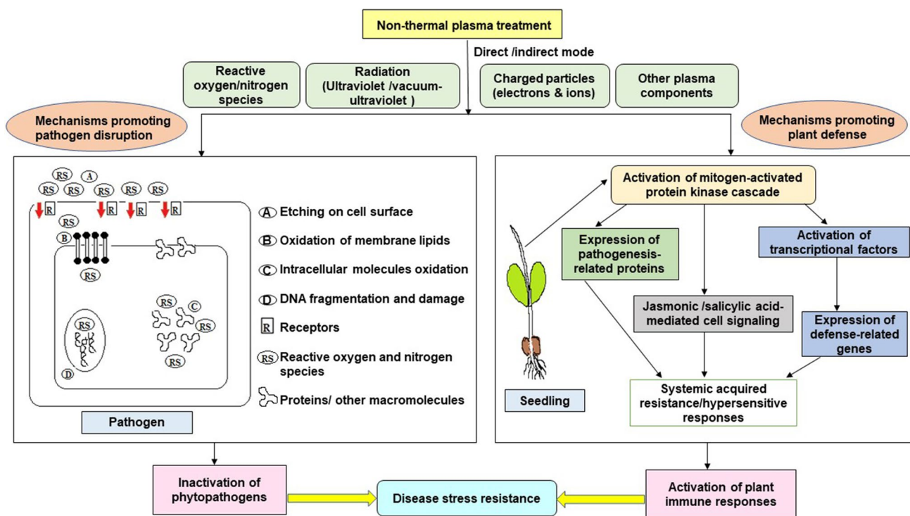
Fig. 3 Putative mechanisms enhancing microbial inactivation and disease stress tolerance in plants through non-thermal plasma treatment. Plasma components initially act to prevent entry of pathogen into the plant cell by etching, degradation of vital proteins and DNA in the cells of microbes. If the pathogen subsides this damage and gain entry into the plant cells, plasma components could possibly trigger defense responses mainly by the activity of reactive species. Reactive species such as NO and H 2 O 2 act as key signaling mol-
