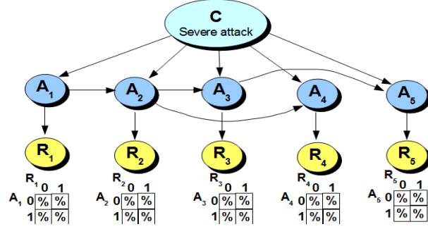
Figure 4: Example of a Bayesian network classifier handling the reliability of inputs
