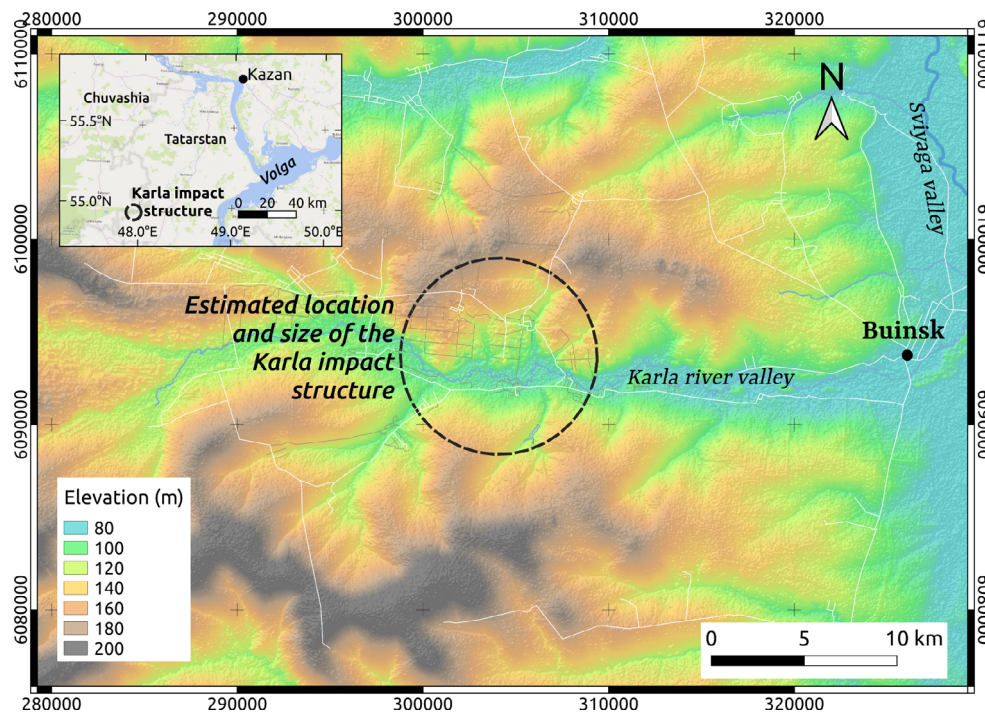
Fig. 1. Topographical map of the Karla impact structure. Inset shows the geographical location of the structure southwest of the city of Kazan. The 30 arc second Shuttle Radar Topography Mission (SRTM) elevation grid was used for elevation. The white lines correspond to the local primary and secondary roads. Coordinates are expressed in meters in the UTM Zone 39U projection with WGS84 datum, except for the inset with geographical coordinates.
