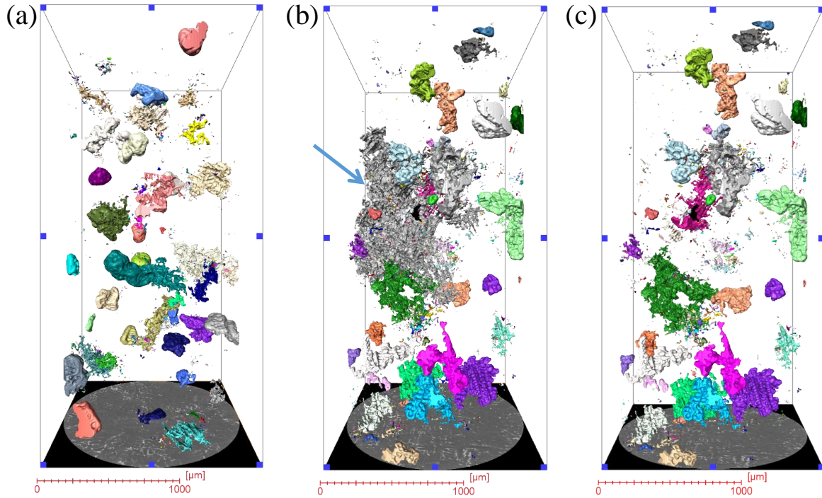
Figure 6: 3D rendering of pores for (a) standard alloy sample, (b) high-Fe/Mn sample and (c) high-Fe/Mn sample without the largest shrinkage
