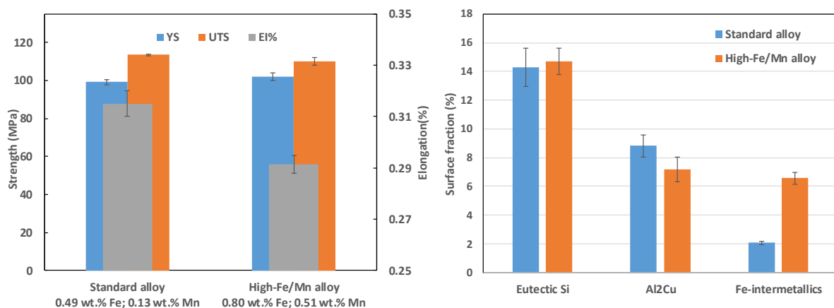
Figure 11 : (a) The tensile properties of the as-cast Al–Si–Cu alloys with different Fe/Mn contents (YS: yield strength; UTS: ultimate tensile strength; El: elongation); (b) Surface fraction of hard inclusions in the fracture surface for standard and high-Fe/Mn specimen.
