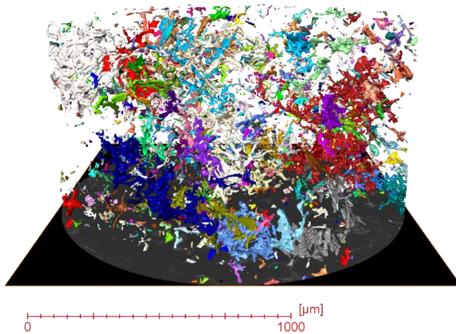
Figure 10: 3D rendering of Al 2 Cu phase for standard alloy
