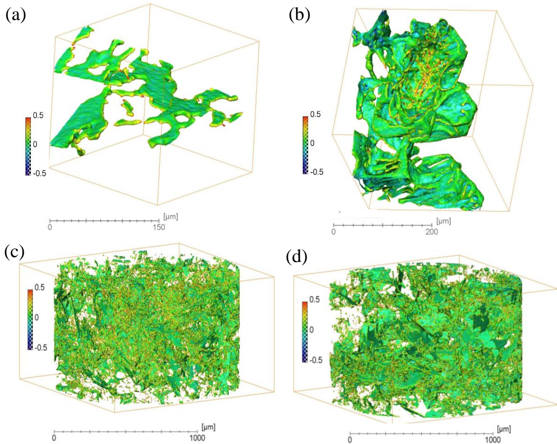
Figure 8: 3D rendering of intermetallics for (a) \beta -Fe, (b) \alpha -Fe, Fe-intermetallics phases in (c) standard and (d) high-Fe/Mn alloy; the colour represents the mean curvature values at the interface location.
