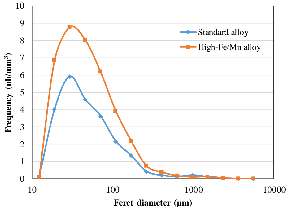
Figure 7: Size distribution of pores in frequency for standard alloy and high-Fe/Mn alloy
