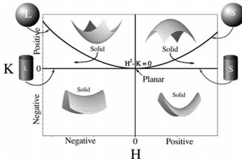
Figure 1: Map of local surface shapes in H-K space [18]
