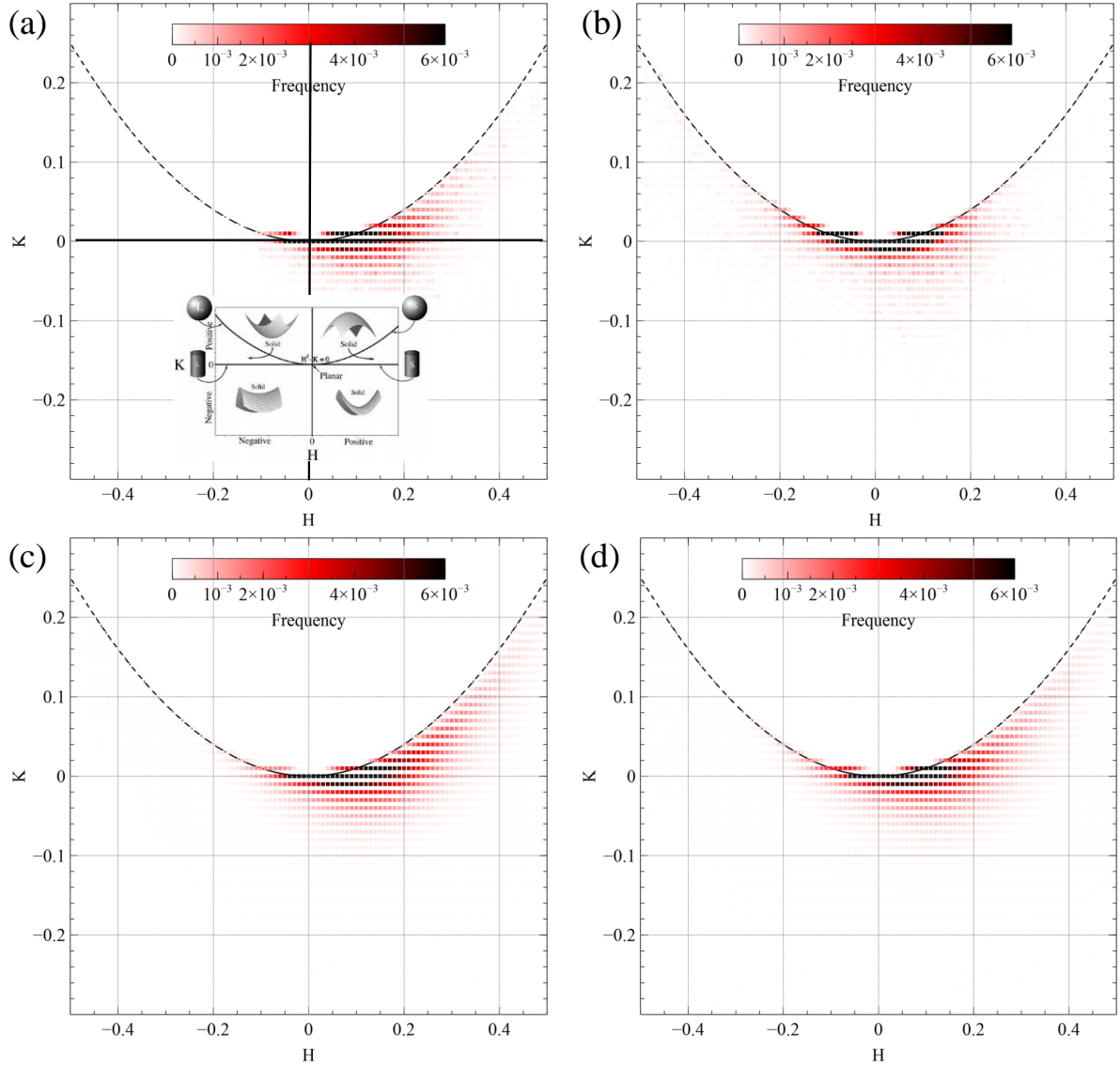
Figure 9: (a), (b), (c) and (d) show the probability density distributions in H-K- coordinates for the microstructures shown in Figure 8 (a), (b), (c) and (d), respectively, i.e. for (a) \beta -Fe, (b) \alpha -Fe, Fe-intermetallics phases in (c) standard and (d) high-Fe/Mn alloy.
