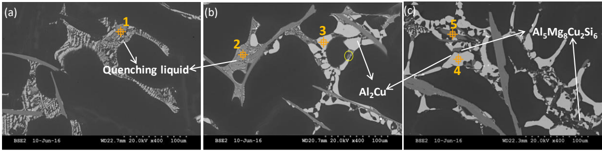
Figure 3: BSE micrograph of the sample quenched at temperature (a) before peak 4 and immediately after (b) peak 4 and (c) peak 5
