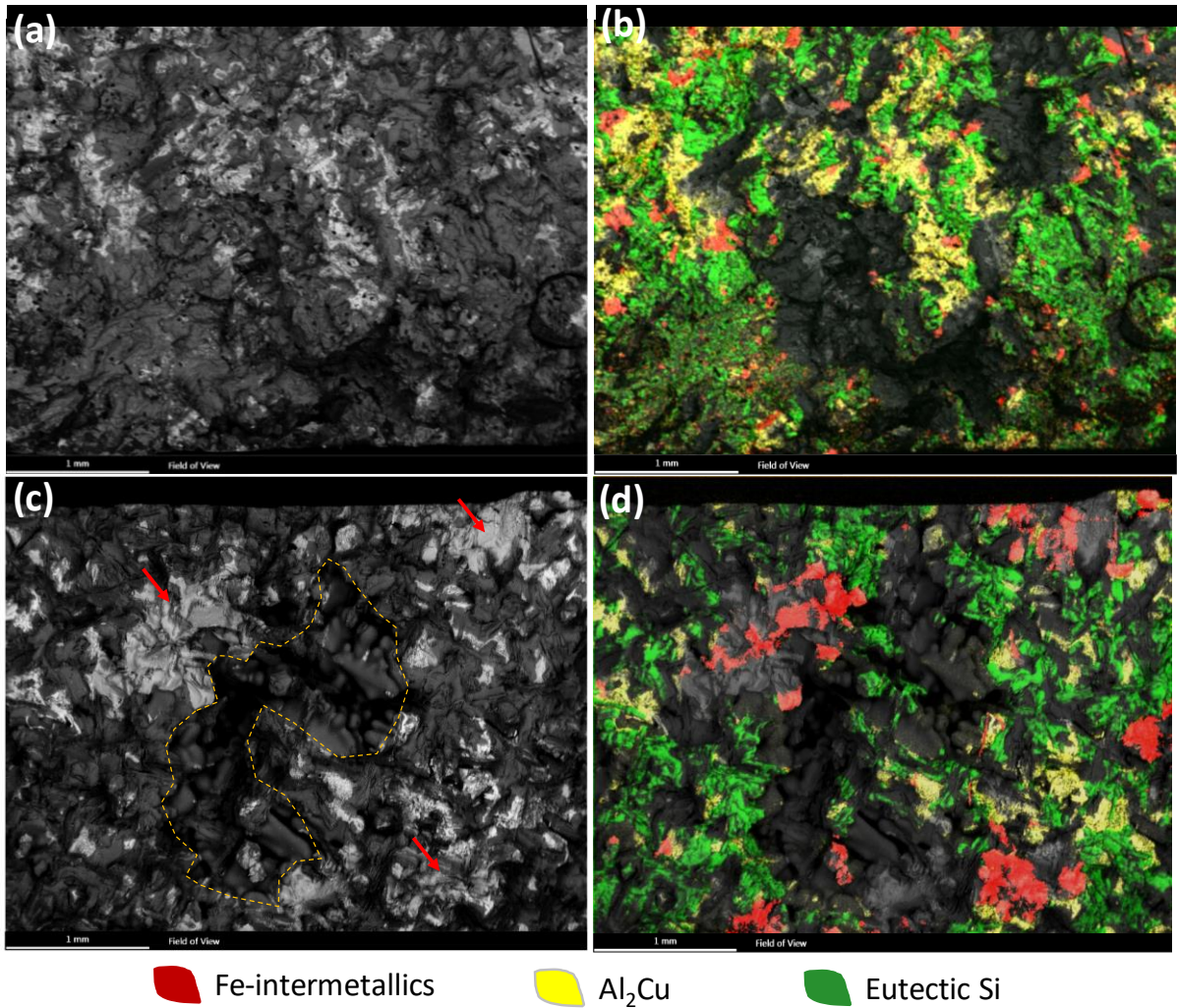
Figure 12 : BSE images of the fracture surfaces and corresponding X-ray mapping images showing the distribution of hard inclusions (eutectic Si, iron-intermetallics, Al 2 Cu phases) of (a, b) standard and (c, d) high-Fe/Mn specimen.
