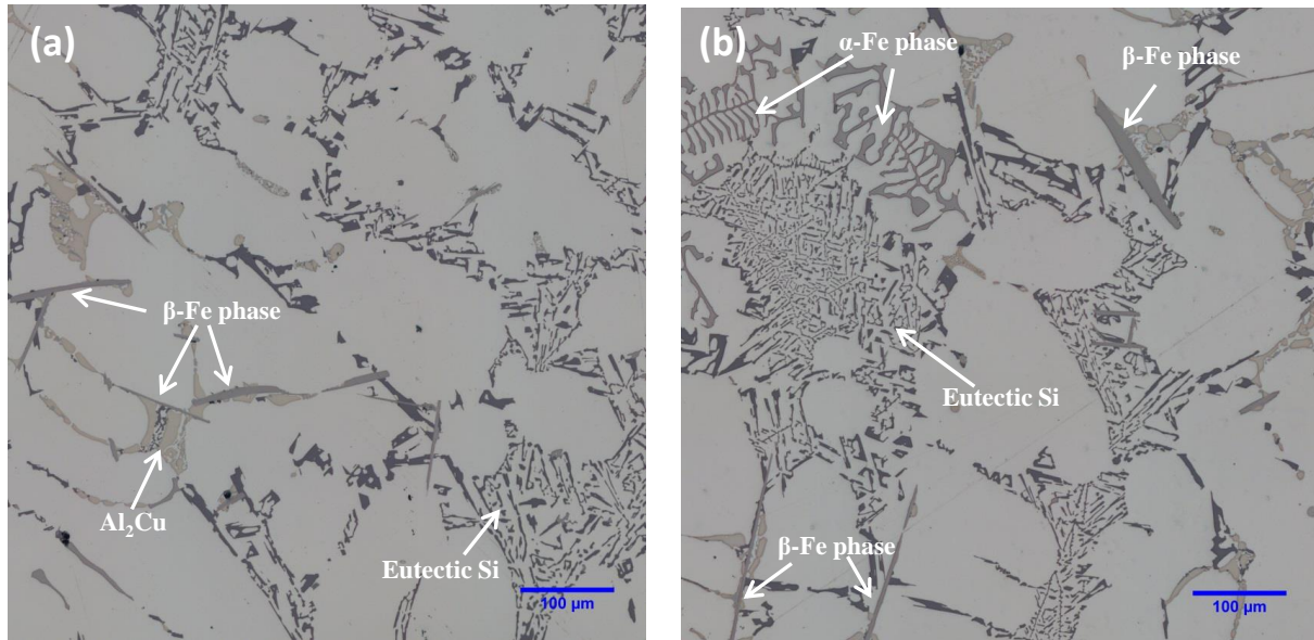
Figure 5: Optical microstructures of sample for (a) standard and (b) high-Fe/Mn alloy
