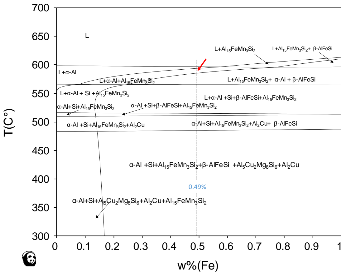
Figure 13: The cross section of equilibrium phase diagram of the studied standard Al-Si-Cu alloy calculated by Pandat software
