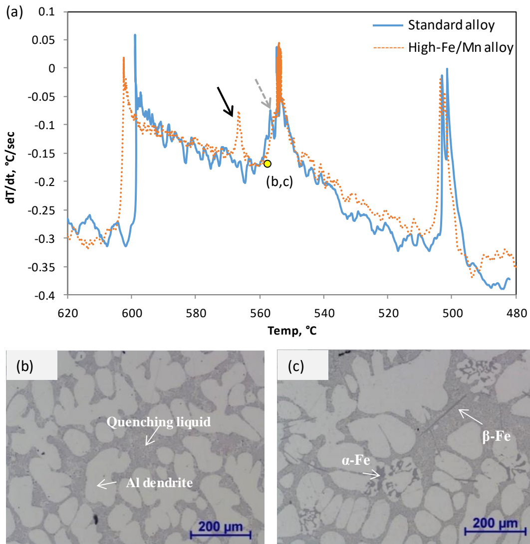
Figure 4: Temperature derivatives measured from the melts with different Fe/Mn addition. Microstructures of samples quenched at 560°C for (b) Standard alloy and (c) High Fe/Mn alloy
