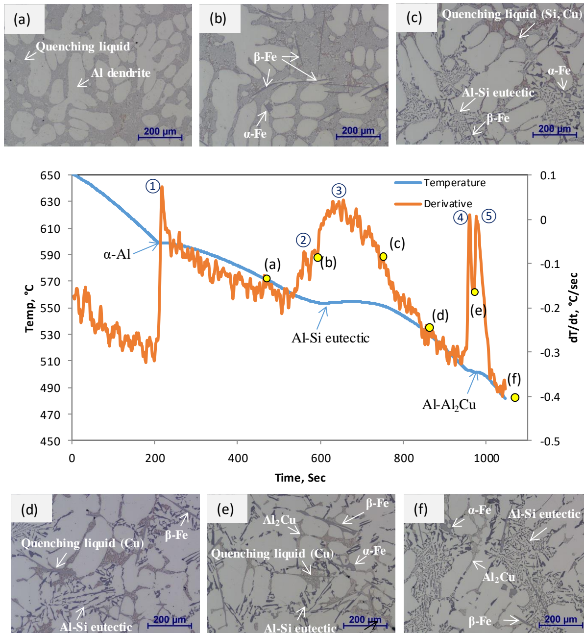
Figure 2: Solidification curve (in blue) and its first derivative (in red) for standard alloy and optical micrograph after interrupted quenching at different temperatures: (a) 560°C, (b) 554°C, (c) 547°C, (d) 520°C, (e) 502°C and (f) full solidification
