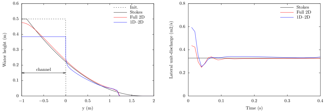
(a) Water height along the y -axis at t = 0.4\text{s}
