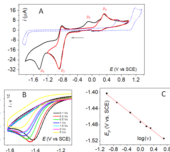
Figure 3 : A: CV of 1.1 mM of \text{Mn}^{\text{II}}(\text{dpaq})(\text{OTf}) in DMF with 0.1 M \text{TBAPF}_6 on glassy carbon electrode with d=0.3 \text{ cm} at v=0.1 \text{ V/s} , T=293 \text{ K} . Argon saturated (blue dotted trace), air saturated (black and red traces, different potential window). B: CVs of the air saturated solution at different scan rates after a 20 second pre-electrolysis at -1.1 V vs SCE. 0.1 V/s (black trace), 0.2 V/s (red trace), 0.5 V/s (light green trace), 1 V/s (blue trace), 1.5 V/s (cyan trace), 2 V/s (violet trace), 5 V/s (yellow trace). C: Variation of the peak potential of p_2 with respect to the scan rate: \partial E/\partial \log v = -59 \text{ mV} .
