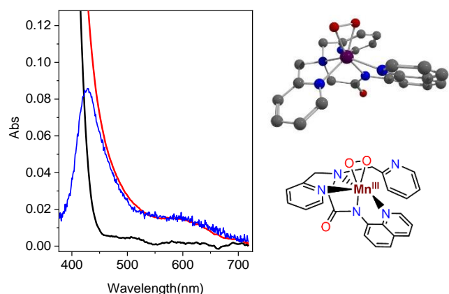
Figure 2 : Left: UV-Vis spectroelectrochemistry of 1.1 mM of \text{Mn}^{\text{II}}(\text{dpaq})(\text{OTf}) in air saturated ( [\text{O}_2] = 1 \text{ mM} ) DMF solution with 0.2 M \text{TBAPF}_6 . WE: Carbon paper. Electrolysis at -1.1 V vs SCE. Optical path 0.1 cm, at 253 K. Black trace: \text{Mn}^{\text{II}} , before electrolysis, red trace: peroxy, after 10 min electrolysis. Blue trace: linear subtraction (non-smoothed). Right: The DFT optimized structure for [\text{Mn}^{\text{III}}(\text{O}_2)(\text{dpaq-py})] is shown on the right. Geometry optimizations were performed with the TPSS functional and the def2-TZVP (Mn, O, and N atoms) and def2-SVP (C and H atoms) basis sets.
