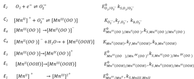
Scheme 4: Equation of the chemical and electrochemical reactions taken into consideration. For the values of the constants see Table S1. Diffusion coefficient for all the Mn species D_{Mn} = 4 \times 10^{-6} \text{ cm}^2 \text{ s}^{-1} , for O_2 4.5 \times 10^{-5} \text{ cm}^2 \text{ s}^{-1} and for superoxide 1.2 \times 10^{-5} \text{ cm}^2 \text{ s}^{-1} . The value of \alpha was taken as 0.5 for all the electron transfers. Initial H_2O was considered to be 30 mM.
