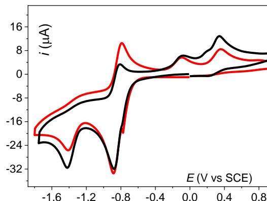
Figure 5: CV of 1.1 mM of Mn^{II}(dpaq)(OTf) in air saturated DMF with 0.1 M TBAPF6 on glassy carbon electrode with d=0.3 cm, at v=0.1 V.s -1 , T=293 K (black trace). Simulation (red trace) taking into considerations the reactions described in scheme 3 with [H_2O] = 30 mM.
