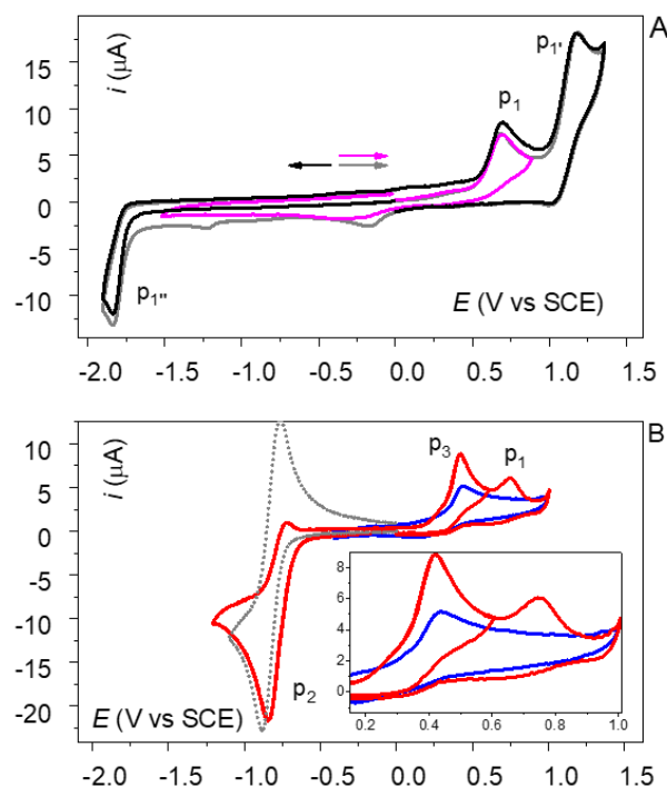
Figure 1 A: CV of 1.1 mM of Mn II (dpaq)(OTf) in argon saturated DMF with 0.1 M TBAPF 6 on glassy carbon electrode with d=0.3 cm at v= 0.1 V/s, T = 293 K, in different potential windows. B: Air saturated solution (red traces, different potential windows) and argon saturated solution after addition of 1.2 eq of KO 2 at 253 K. The O 2 /O 2 •- is shown as grey dotted trace for comparison. Inset: zoom of the p 1 and p 3 oxidation peaks
