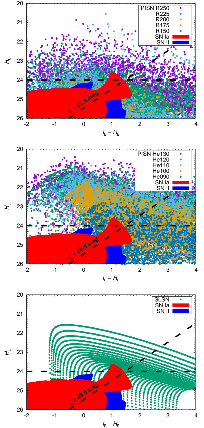
Fig. 12. Color-magnitude diagrams in the I_E and H_E bands for RSG PISNe (top), WR PISNe (middle), and SLSNe (bottom). PISNe and SLSNe at z > 0.5 at all phases are plotted with a redshift interval of 0.1. The color evolution with time can be found in Fig. 13. The regions covered by SNe Ia and SNe II at z > 0.5 are shown. No extinction is assumed. The survey limiting magnitudes for the I_E and H_E bands (25.5 mag and 24.0 mag in AB magnitudes, respectively) are indicated by the dashed lines. Most SNe Ia and SNe II at z > 0.5 are too faint to be detected in the H_E band with the 24.0 mag limit.
