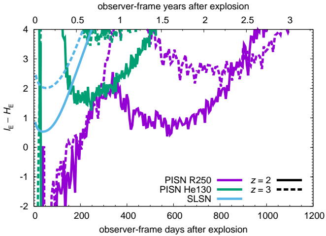
Fig. 13. Color evolution of the PISN models and SLSN template presented in Fig. 3.
