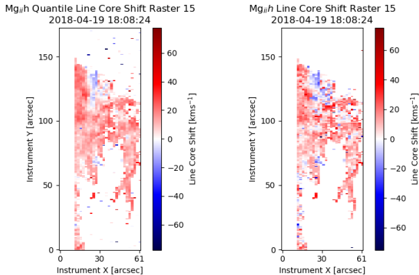
Fig. 19. Comparison of line core shift recovered by quantile method and rolling RMS procedure. Left: line core shift recovered by quantile method. Right: line core shift recovered by rolling RMS procedure.
