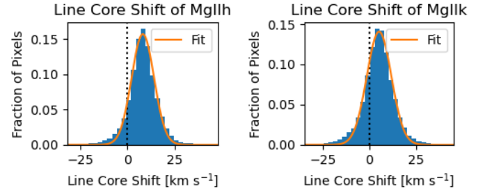
Fig. 8. Line core shift histograms of both Mg II h&k across all 18 rasters with Gaussian fits.
