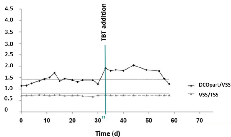
Figure 7. Evolution of VSS/TSS and CODpart/VSS ratios in MBRi system.
