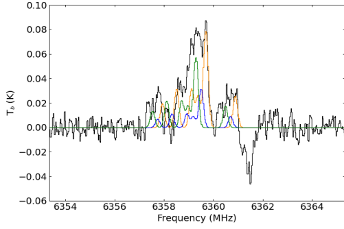
Fig. 3. Illustrative spectrum of \text{CH}_3\text{CONH}_2 showing the relative intensities of all the HFS (Table 6) and multiple velocity components at +62 (in yellow), +71 (in blue) and +81 km s -1 (in green) overlaid on the GBT spectrum of Sgr B2(LMH) (in black). The intensity of these emission features cannot be matched by the synthetic LTE model in this work.
