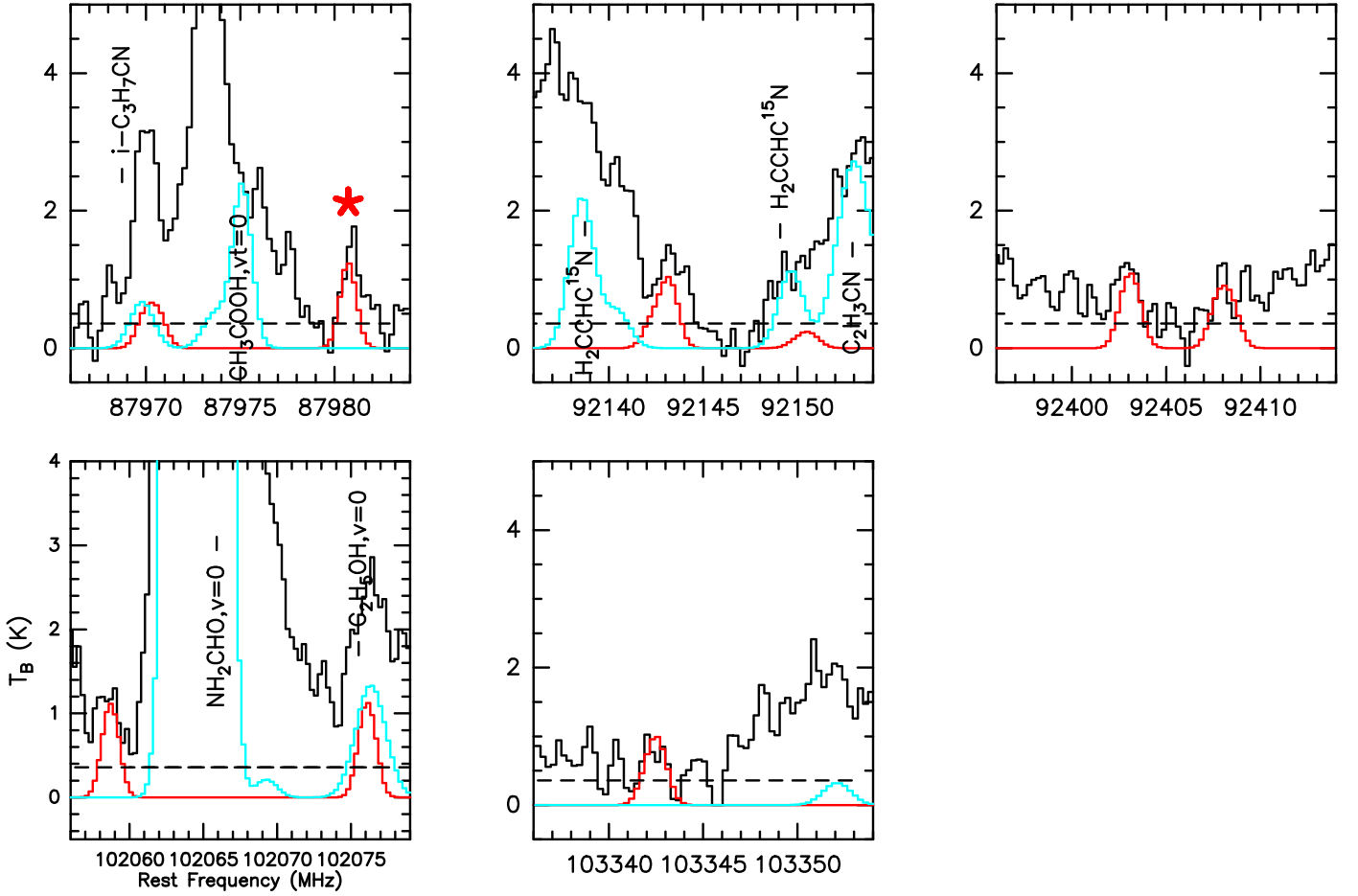
Figure 5. Clean transitions of C_2H_5CONH_2 v=0 toward Sgr B2(N1E). Continuum-subtracted spectrum observed with ALMA in black, the synthetic spectra of C_2H_5CONH_2 in red, and the preliminary model of other identified molecules in cyan. Red star denotes the 87,980 MHz line that has been detected with IRAM 30 m. The dashed lines denote the 3\sigma levels ( \sigma ranges from 0.12 to 0.4 K). The observed data behind these figure panels are available.
