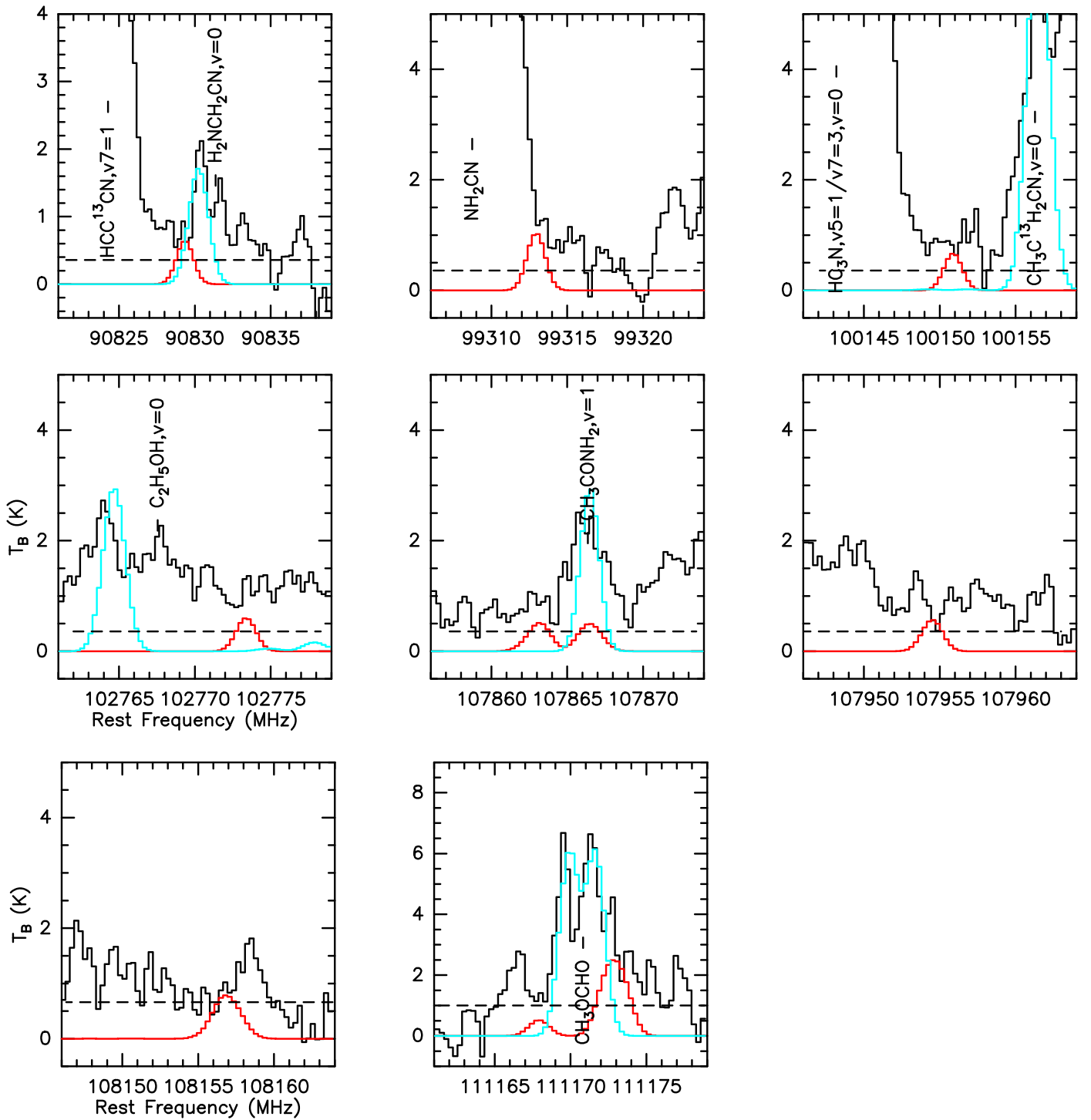
Figure 7. Partially blended transitions of \text{C}_2\text{H}_5\text{CONH}_2 v=1 detected with the ALMA telescope toward the Sgr B2(N1E). See caption of Figure 5 for more detail. The observed data behind these figure panels are available.
