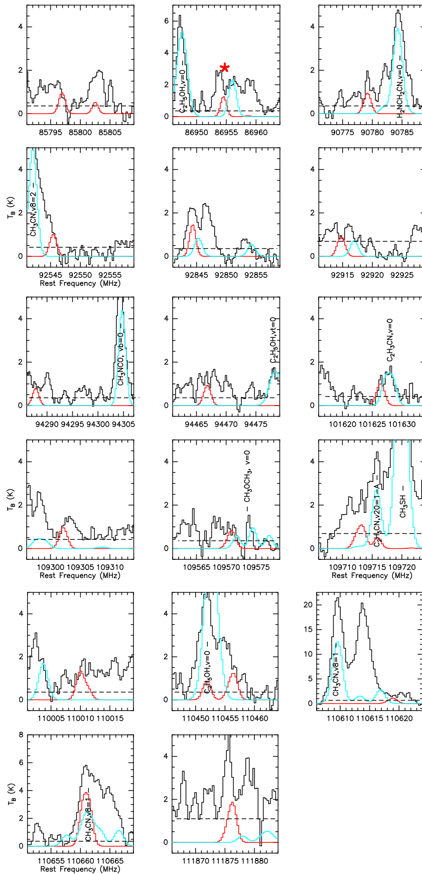
Figure 6. Partially blended transitions of C_2H_5CONH_2 v = 0 detected with the ALMA telescope toward the Sgr B2(N1E). See caption of Figure 5 for more detail. The observed data behind these figure panels are available.
