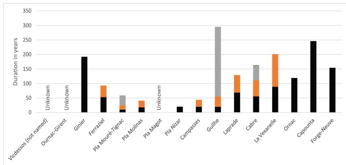
Fig. 6 : Evaluation of the maximum running duration for each bloomery (colors correspond to successive phases of activity).
