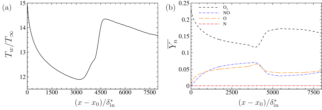
Fig. 23. Streamwise evolutions of (a) normalized wall temperature and (b) mean mass fractions \bar{Y}_n along the wall. In panel b, \bar{Y}_{N_2} is not shown being outside of the prescribed range.
