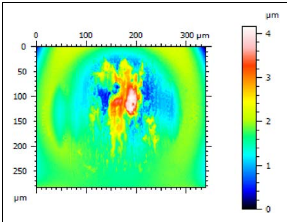
Figure 17. Ball scar.
