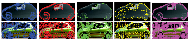
Fig. 5: Features extracted in the depth (row 1) and the real image (2) with: MCS (column 1), PCI proposed in [8] (2), SIFT (3), Harris (4) and Edge detector proposed in [12] (5).
