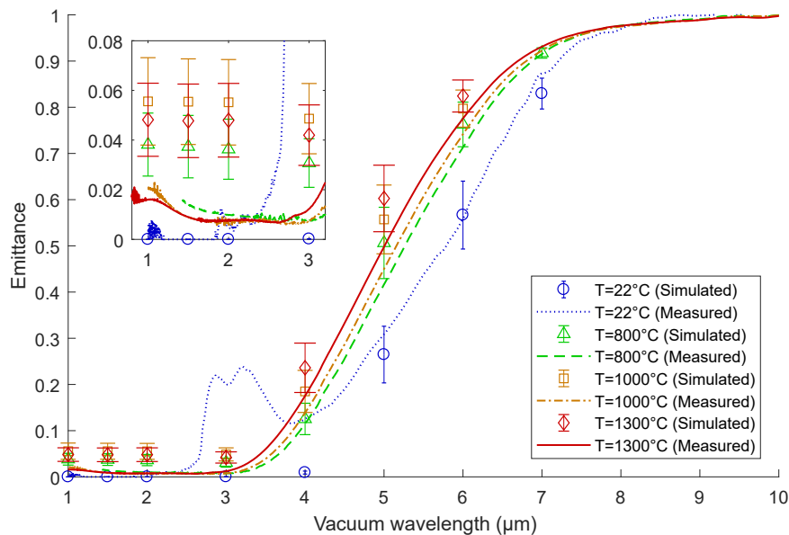
Figure 6: Measured (lines) and simulated (symbols) spectral normal emittance of the porous alumina disks at different temperatures T : 22 °C (dotted lines vs. \circ ), 800 °C (dashed lines vs. \Delta ), 1000 °C (dash-dotted lines vs. \square ), 1300 °C (continuous lines vs. \diamond ). The inset shows the near-zero emittances at wavelengths between 1 \mu\text{m} and 3 \mu\text{m} .
