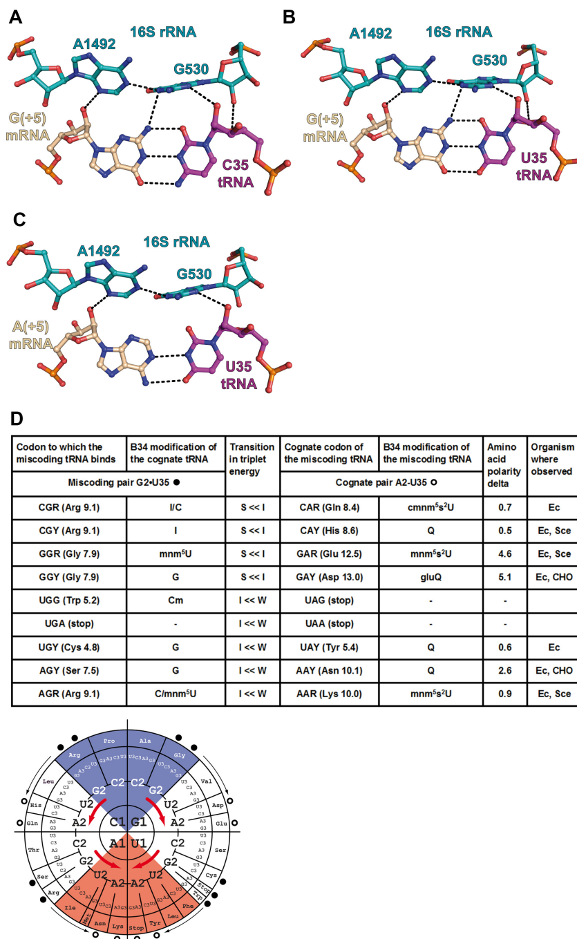
Figure 4. Substitution of a G2 = C35 pair or an A2-U35 pair by a G2•U35 base pair in the second position of the codon-anticodon duplex. (A) Cognate G2 = C35 pair from the complex of 70S ribosome with mRNA and tRNA Arg (this study, PDB ID: 6gsl); (B) near-cognate G2•U35 pair from the complex of 70S ribosome with mRNA and tRNA Tyr (PDB ID: 4v8e); (C) A2-U35 pair from the complex of 70S ribosome with mRNA and tRNA Lys (PDB ID: 5e7k). The nucleotides of the 16S rRNA are depicted in teal, tRNA in magenta and mRNA in wheat. The dashed lines indicate the putative hydrogen bonds (interatomic distance \leq 3.3\text{\AA} ). (D, top) Summary table of all amino acid substitutions resulting from the incorporation of the mismatched pair with comparisons of amino acid polarity, transition in triplet energy between the two cognate tRNAs (S = Strong, I = Intermediate, W = Weak), the experimentally observed G•U pairing miscoding available in the literature ( Escherichia coli (EC), Saccharomyces cerevisiae (Sce) and CHO cells). The in vivo data for E. coli and S. cerevisiae are from (6,7) and (28); those for the CHO cells are from (27). The transition in triplet energy between cognate tRNAs and the base modification at nucleotide 37 in the respective cognate tRNAs (for E. coli ) are both indicated to point to the competition between the tRNAs for the A site. The cognate codon of the miscoding tRNA is at the right and at the left the miscoding pair formed by the miscoding tRNA. (D, bottom) The corresponding tRNA modifications and relative positions of cognate and near-cognate codons on the energy wheel. The miscoding pairs (dark circles) are indicated with the thin arrows pointing to the miscoding tRNA (open circles) (e.g. a tRNA His miscodes an Arg codon or a tRNA Asp miscodes a Gly codon). The thick red arrows indicate the energetic transitions between Strong (blue) and Intermediate (white) codon-anticodon triplets as well as between Intermediate and Weak (red) ones. Because the substitutions are at the second position, the transitions occur within each of the four quadrants. The miscoding tRNAs are highly modified and replace stronger, but less modified, tRNA binders. Many instances have been reported in the literature.
