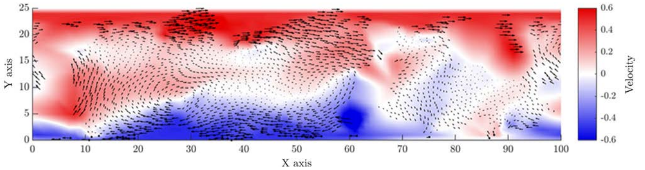
Fig. 6 Velocity vector of each particle in the simulation at time T = t + 2\Delta t (black arrows), and interpolated velocity field from the particle velocities (colored field)
