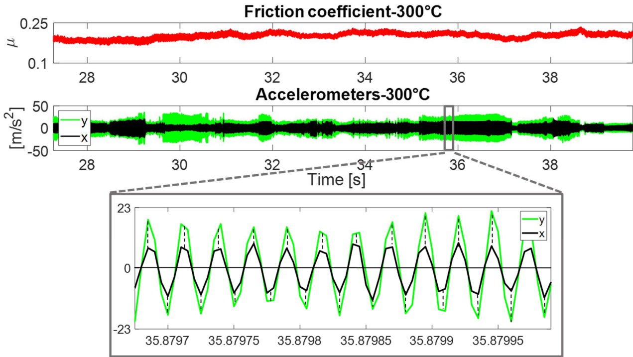
Figure 11. Detail of the friction coefficient and vibrational response of a single stroke at 300°C and in the constant sliding velocity test ( V=3 mm/s). From the top: friction coefficient and accelerometer signals along the tangential ( X ) and normal ( Y ) direction to the contact.
