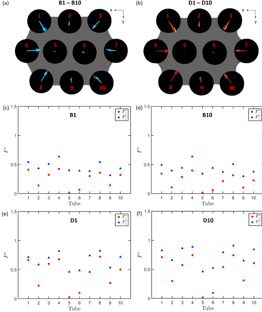
Figure 7. (a,b) Cross sections of the fibre network showing the transverse capillary force F_{\perp} exerted by the fluid on each tube (in black) for stages B_1 (dark blue arrows) and B_{10} (pale blue arrows) and D_1 (red arrows) and D_{10} (yellow arrows) of the impregnation experiment carried out with the demineralised water. The application points of the forces were placed arbitrarily on the axes of the tubes. The cross section of the fibre network was also chosen arbitrarily (the fluid is grey in the cross section). Graphs showing the dimensionless transverse F_{\perp}^* and longitudinal F_{\parallel}^* capillary forces exerted by the fluid on each tube for stages B_1 (c), B_{10} (d), D_1 (e) and D_{10} (f).
