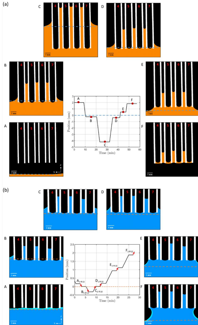
Figure 3. Vertical cross sections of the 3D images acquired during the impregnation of the fibre network with silicone oil (a) and demineralised water (b). The dashed lines show the initial position of the fluid surface. The tubes are represented in white, the air in black, the silicone oil in orange and the demineralised water in blue. The graphs represent the position of the bottom extremities of the tubes with respect to the initial position of the fluid surface as a function of time. The red arrows in the graph indicate the time intervals when the sequences of 3D images were acquired
