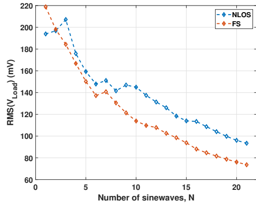
Fig. 5: DC voltage (RMS value) of the designed waveforms collected at the output of the energy harvesting circuit as a function of N for NLOS and FS scenarios.
