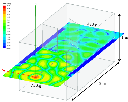
Fig. 2: 3D electromagnetic model: Reader and tag antennas separated by an NLOS propagation environment.
