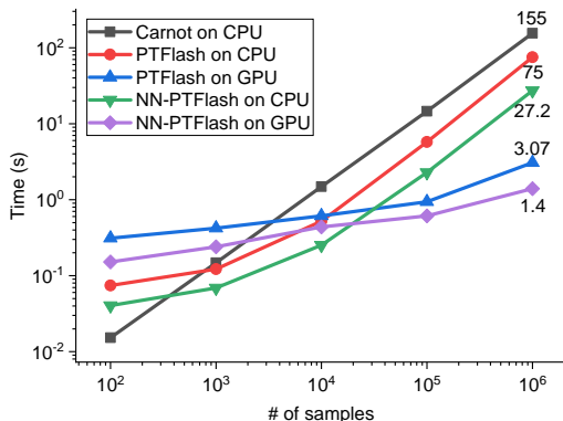
(c) Mixture of 9 components
