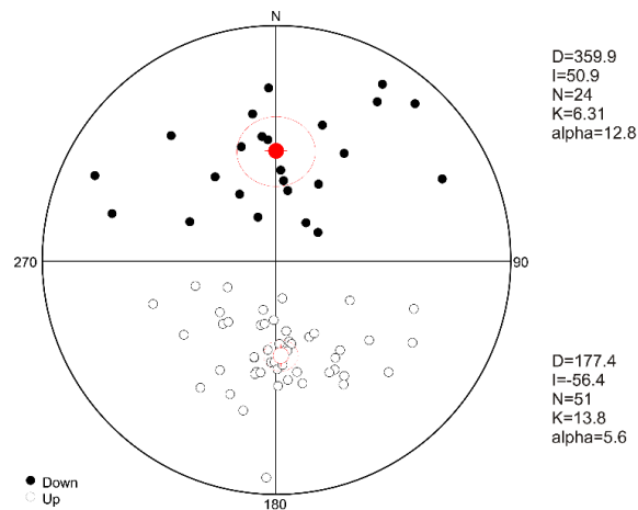
Figure 5. Stereographic projection of characteristic directions (normal and reversed polarities) isolated from the studied samples. Red dot is the calculated mean direction, while the red circle around it represents the 95% confidence limit [41]. D, I and alpha in degrees (°).
