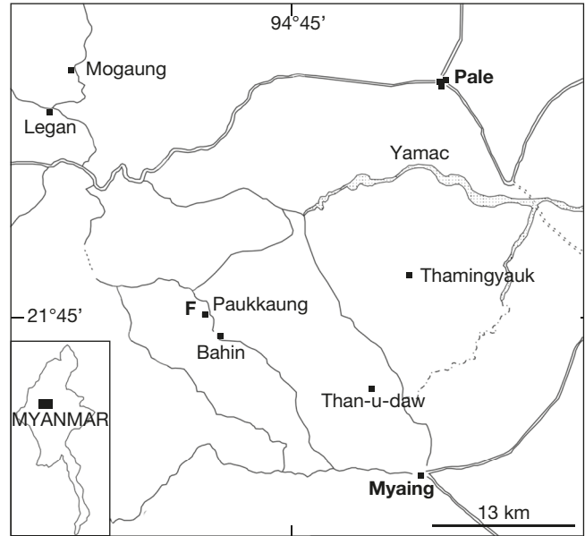
FIG. 1. — Location map of the Pondaung area. F indicates Paukkaung 2 locality.
