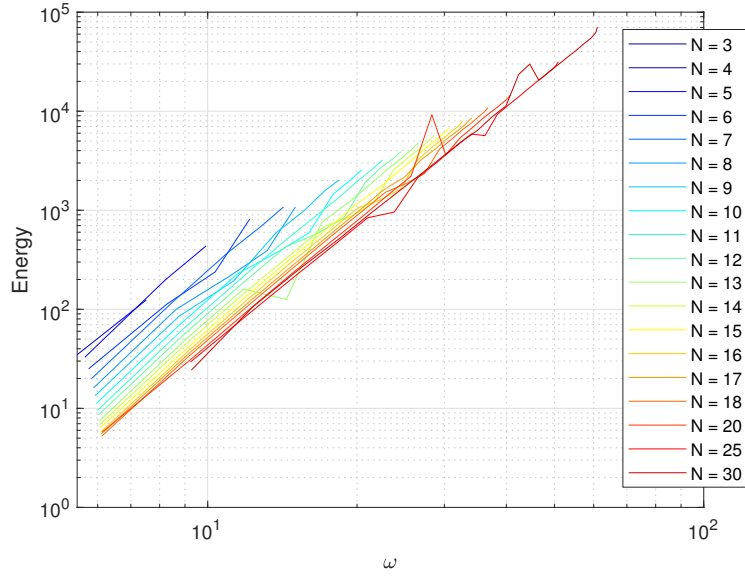
Figure 17: Energy of the first bifurcation of each mode for several values of N in logarithmic scales.
