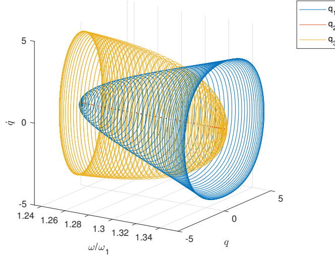
Figure 10: Phase diagram along the secondary branch between non-linear modes 1 and 3.
