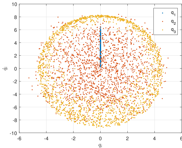
Figure 14: Section of Poincaré between 2000 and 10000 s of the Hamiltonian system for initial energy of 50 on mode 2.
