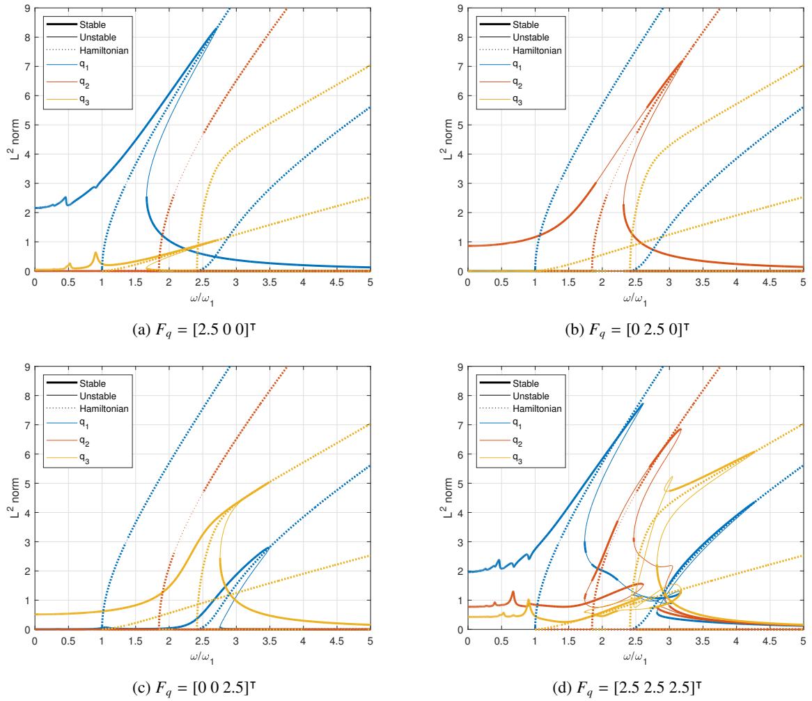
Figure 7: Response of the system ( N = 3 ) with \lambda = 0.01 and an excitation on each eigenmode computed with HBM ( H = 20 ).
