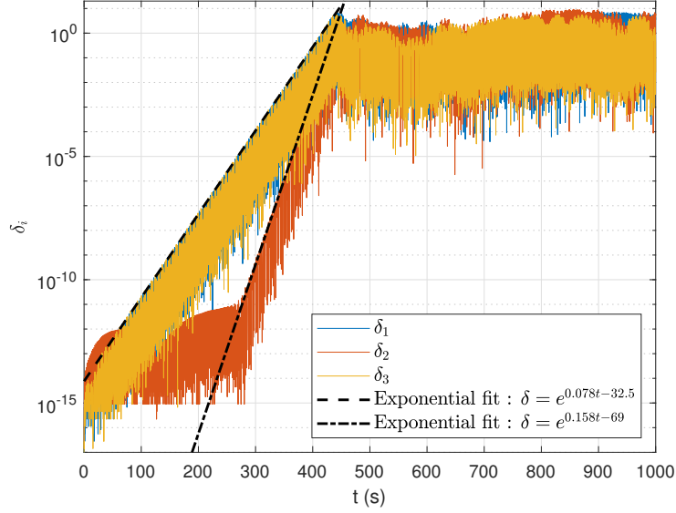
Figure 15: Difference between the modal coordinates of two responses with very close initial conditions.
