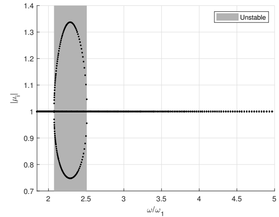
(d) Norm of Floquet multipliers for the second non-linear mode.
