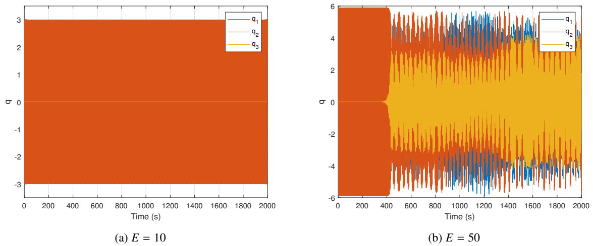
Figure 13: Response of the Hamiltonian system for several values of initial energy on mode 2.
