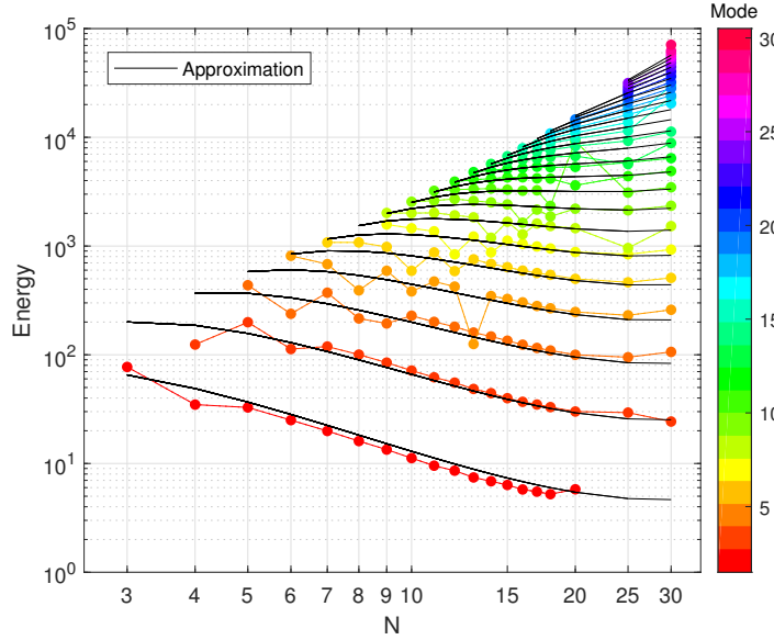
Figure 18: Energy of the first bifurcation of each mode for several values of N in logarithmic scale.
