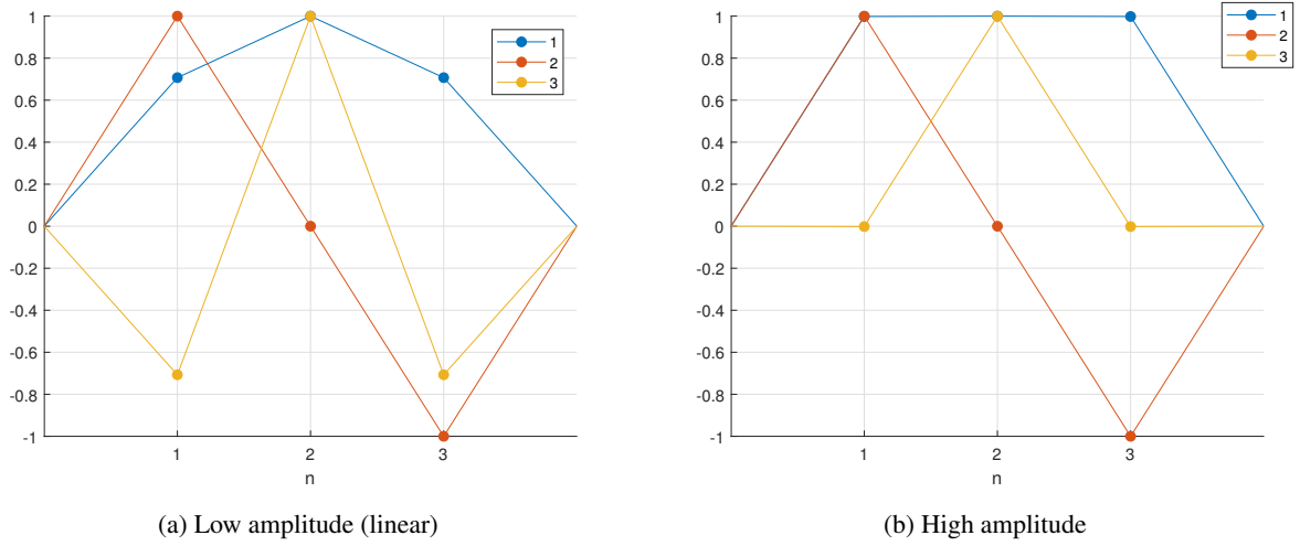
Figure 5: Shape of the non-linear modes normalized with maximum value for very low amplitude and very high amplitude on each branches for N = 3 .
