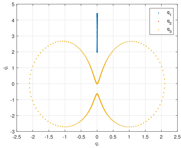
Figure 12: Poincaré section for the time response in Fig. 11d.
