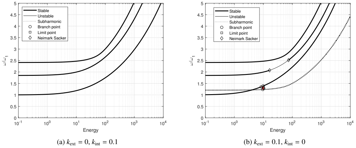
Figure 8: Frequency-energy plot for N = 3 .
