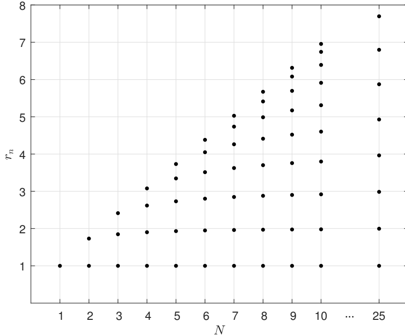
Figure 2: Frequency ratios r_n = \frac{\omega_n}{\omega_1} of the system for several values of N .
