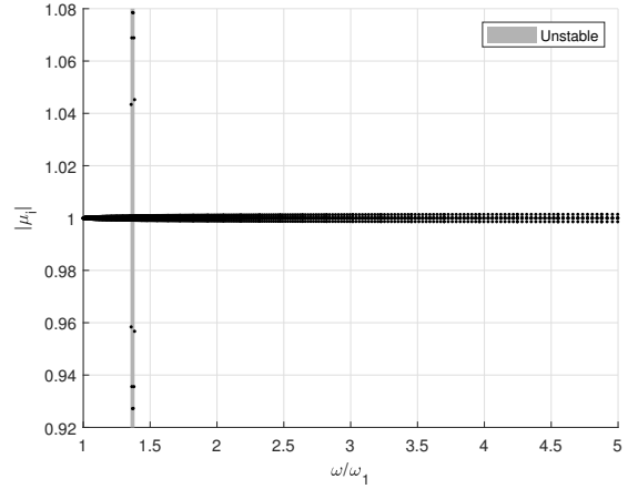
(b) Norm of Floquet multipliers for the first non-linear mode.
