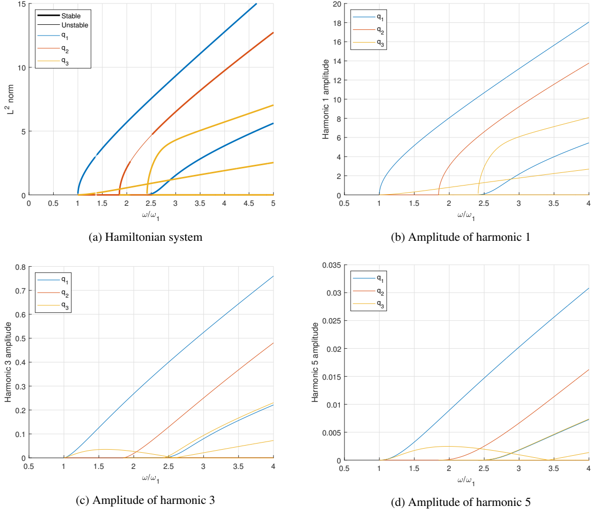
Figure 3: Non-linear normal modes and significant harmonics (1, 3 and 5) with H = 20 .
