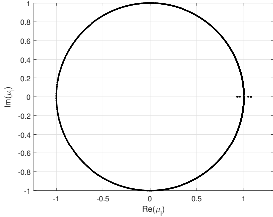
(a) Floquet multipliers in complex plane for the first non-linear mode.
