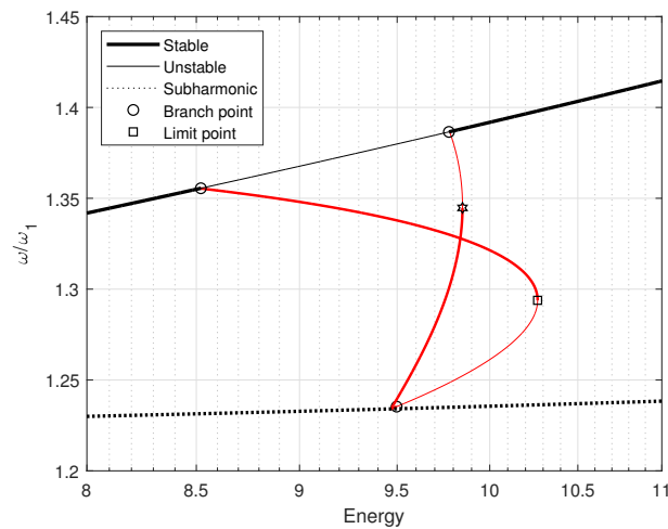
Figure 9: Zoom of Fig. 8b. Secondary branch between non-linear mode 1 and subharmonic of the non-linear mode 3.
