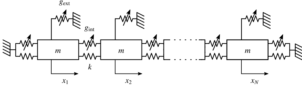
Figure 1: Chain of N non-linear oscillators.
