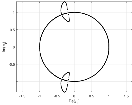
(c) Floquet multipliers in complex plane for the second non-linear mode.
