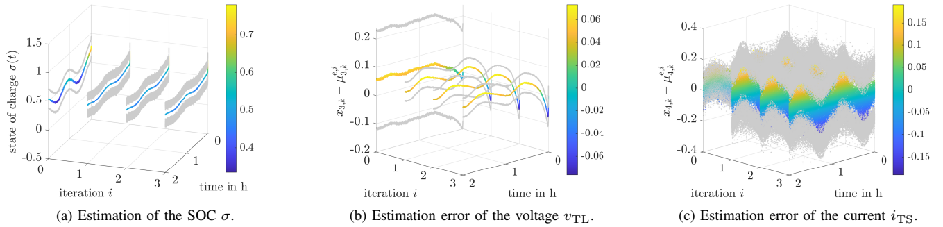
Fig. 4: Estimation results of the stochastic ILO in the Case C2 with \pm 1 standard deviation bounds in gray color (new ellipsoidal covariance prediction), where the iteration 0 corresponds to the pure along-the-trial estimates.
