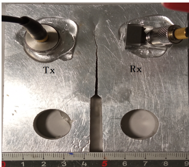
Figure 3: Cracked sample. Transmitter on the left, receptor on the right.
