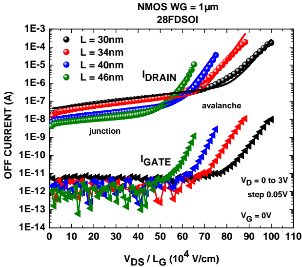
Figure 15: I_{DS} and I_G measurements and modeling at T = 125^\circ\text{C} under Off-state ( V_{GS} = 0 ) for L_G = 30\text{nm} to 46\text{nm} NFETs as a function of peak lateral field approximated to E_{max} \approx V_{DS} / L_G showing a junction leakage and avalanche components in the diode currents. The modeling is shown in lines for I_{DS} monitoring with relatively good agreements as a function of gate-length L_G .
