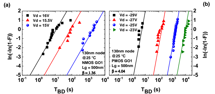
Figure 7: Time to breakdown distribution plots for GO1 W_G/L_G = 10\mu\text{m}/500\text{nm} 130nm FET at 25 °C and various drain voltage V_{DS} (a) in NMOS with lower \beta and (b) in PMOS devices.
