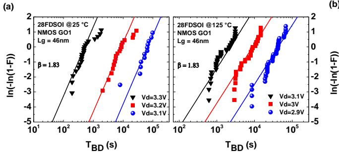
Figure 5: Cumulative distribution with same Weibull slope obtained in GO1 W_G/L_G = 1\mu\text{m}/46\text{nm} 28FDSOI NFET at various stressing drain bias between (a) 25 °C and (b) 125 °C.
