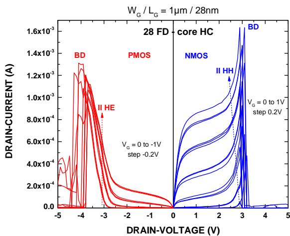
Figure 2: I_{DS} measurements until breakdown as a function of V_{DS} with variables V_{GS} in W_G / L_G = 1\mu\text{m} / 28\text{nm} FDSOI during Off-state and subthreshold conditions. Impact ionization current is higher in NFET than in PFET under same reverse bias and BD occurs around 3V in NFET with HH injection while it seems to reach -4V with HE injection before dielectric BD in PFET.
