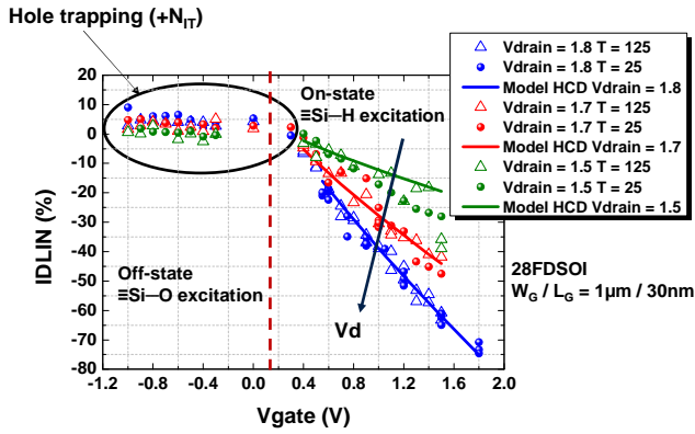
Figure 4: \Delta I_{D,lin} ( V_d = 50 mV) in 28FDSOI N-channel L_G = 30 nm extracted at t_s = 10^4 s. V_g dependence of \Delta I_{D,lin} under HCD in On and Off modes with V_g stress between -1 and 1.8 V with the modeling (lines) in On mode between room temperature (25 °C) and T = 125 °C.
