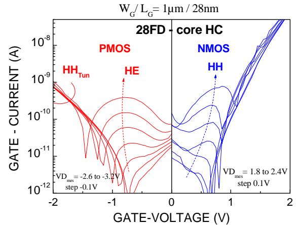
Figure 3: Consequence of Impact Ionization shown in NFET and PFET W_G / L_G = 1\mu\text{m} / 28\text{nm} FDSOI under HC mode seen by gate current ( I_{gate} ) measurements in thin gate-oxide for V_{DS} and V_{GS} variables, showing the distinct injection mechanisms between hot-electrons and hot-holes at low V_{GS} which turns around to a single tunneling component at high V_{GS} .
