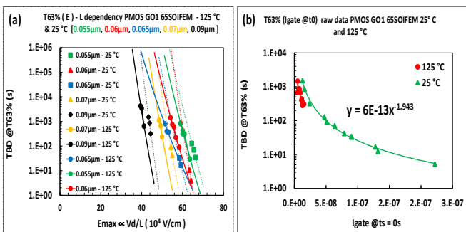
Figure 12: Lifetime plots as t_{BD} at 63% for 65nm PFET (a) vs. electrical field E_{max} \equiv V_{DS}/L_G enlightening L_G dependence between 25°C and 125°C (dashed lines) and 125°C (solid lines) and (b) vs. gate oxide initial leakage current overcoming L_G dependence between 25°C and 125°C.
