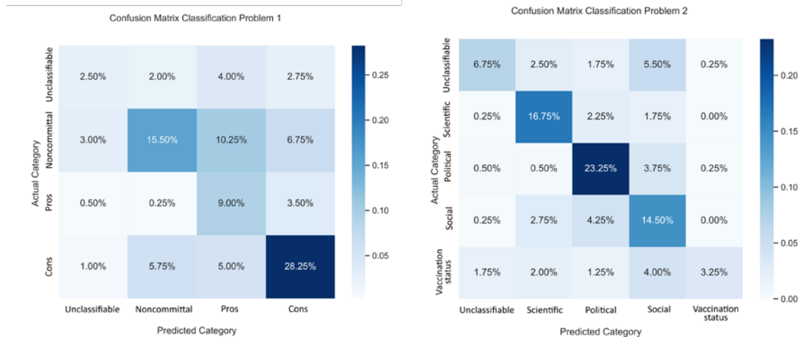
Figure 3: Confusion matrix for classification problems 1 and 2 (N=400).
