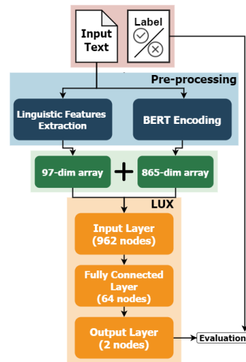
Figure 1: Outline of LUX classifier
