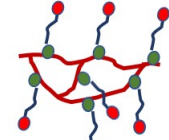
Reticulated polymers
