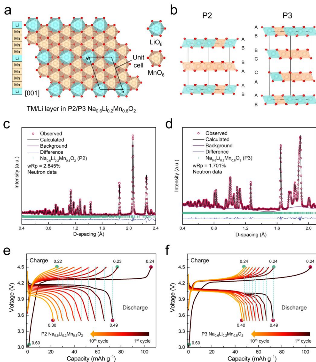
Fig. 1| Ribbon-ordered structure and electrochemistry of P2- and P3- \text{Na}_{0.6}\text{Li}_{0.2}\text{Mn}_{0.8}\text{O}_2 cathode materials. a , Ribbon-ordered structure ( \cdots\text{-Li-4Mn-Li}\cdots ) of the TM layer. b , Illustrations of P2- and P3-type structures. c,d , Refinement results of the neutron diffraction data of P2- and P3-NLMO samples using the structural model from DFT calculations, in which the red dots represent the experimental pattern; black line the calculated pattern; purple line the background curve; blue line the difference curve; green bars the Bragg reflections. e,f , Capacity–voltage curves of ten cycles for P2- and P3-NLMO in a Na half-cell, with the Na content ( x ) near the green or red circle at various states of charge or discharge in \text{Na}_x\text{Li}_{0.2}\text{Mn}_{0.8}\text{O}_2 .
