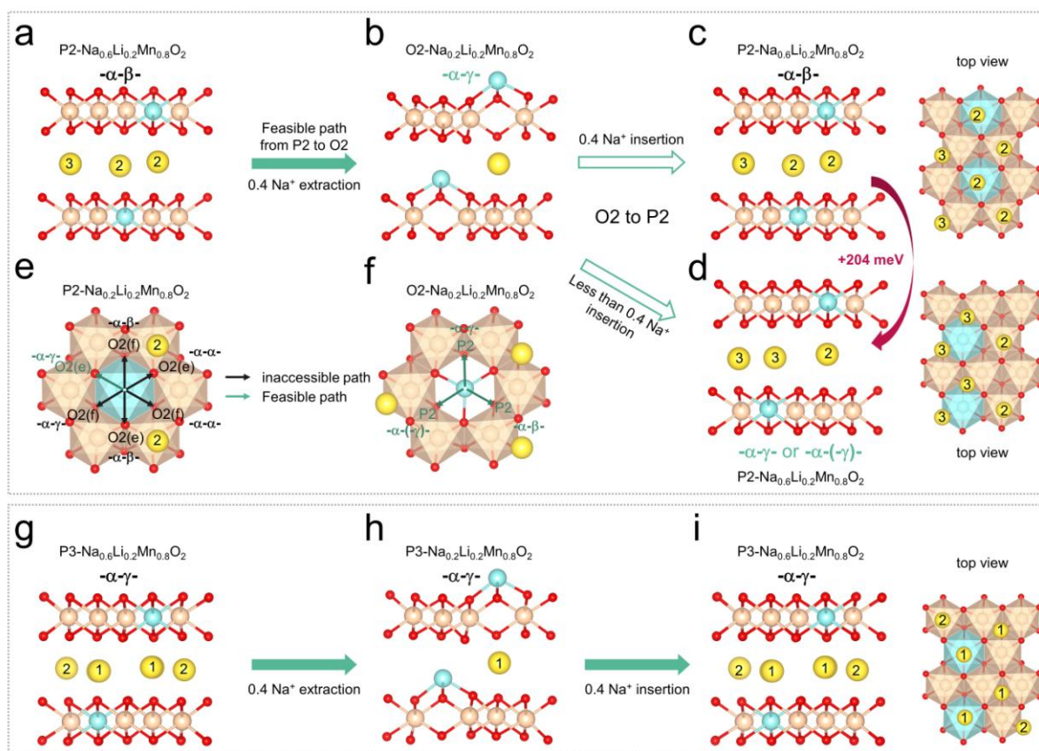
Fig. 4| Topological protection mechanism during Na-ion deintercalation. P2-type: a , Pristine P2-NLMO structure with the - \alpha - \beta - sequence. b , \text{O}_2\text{-Na}_{0.2}\text{Li}_{0.2}\text{Mn}_{0.8}\text{O}_2 structure with the - \alpha - \gamma - sequence at the state of charge of 4.5 V. c , P2-NLMO structure with the - \alpha - \beta - sequence at the state of discharge of 3.5 V (the top view is shown in the right panel). d , P2-NLMO structure with the - \alpha - \gamma - sequence at the state of discharge of 3.5 V (the top view is shown in the right panel). e , glide paths from the P2 structure to O2 structure (a \rightarrow b). f , glide paths from the O2 structure to P2 structure (b \rightarrow c or d). P3-type: g , pristine P3-NLMO structure with the - \alpha - \gamma - sequence. h , \text{P3-Na}_{0.2}\text{Li}_{0.2}\text{Mn}_{0.8}\text{O}_2 structure with the - \alpha - \gamma - sequence at the state of charge of 4.5 V. i , P3-NLMO structure with the - \alpha - \gamma - sequence at the state of discharge of 3.5 V (the top view is shown in the right panel). The cyan ball is the Li ion, the brown ball the Mn ion, the yellow ball the Na ion, and the red ball the O ion. The number of Na ions represents the type of Na ions, as shown in Supplementary Fig. 9.
