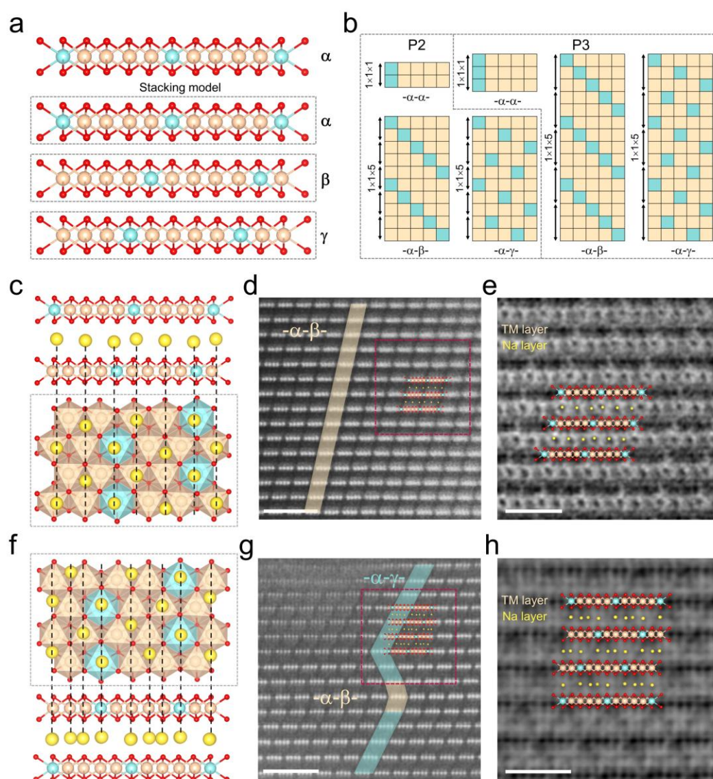
Fig. 2 | One-dimensional topological (ODT) structures and Na configurations in pristine P2- and P3-NLMO. a , Three stacking models of the TM layer including -\alpha-\alpha- , -\alpha-\beta- , and -\alpha-\gamma- sequences. b , ODT structures of P2- and P3-NLMO induced by the stacking models, with the cyan and brown boxes representing the Li and Mn ions in the TM layer, respectively. P2-type: c , Optimized structure (side and top views). d,e , HAADF- and ABF-STEM images (the inset shows the optimized P2 structure). P3-type: f ,
