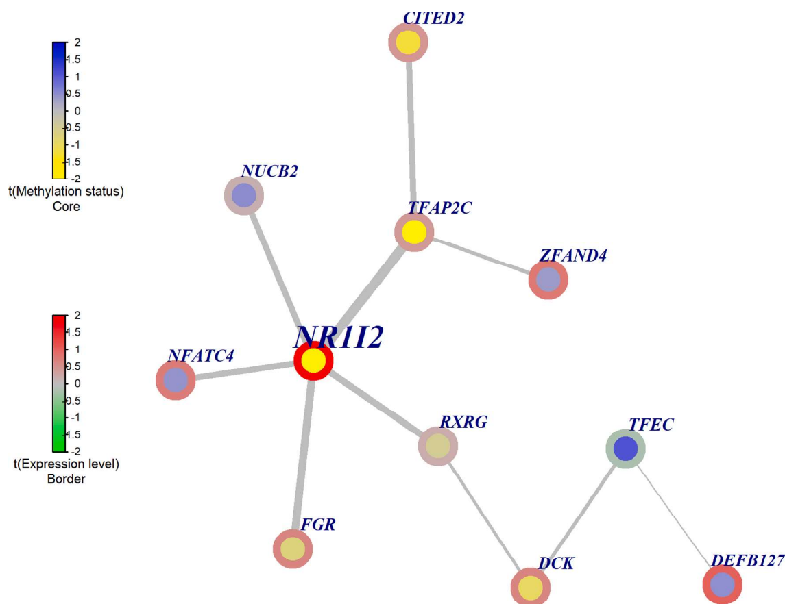
Fig. 2. Top statistically significant functional epigenetic module around seed gene NR112 related to PM 2.5 exposure at birth address. The color of node represents the DNA methylation status. Blue represents hypermethylation, whereas yellow represents hypomethylation. The different color of border refers to the expression patterns. The red color of border represents that the genes were upregulated, whereas the green color of border represents that the genes were downregulated. Edge widths are proportional to the average statistic of the gene-gene interaction network. (For interpretation of the references to color in this figure legend, the reader is referred to the web version of this article.)
