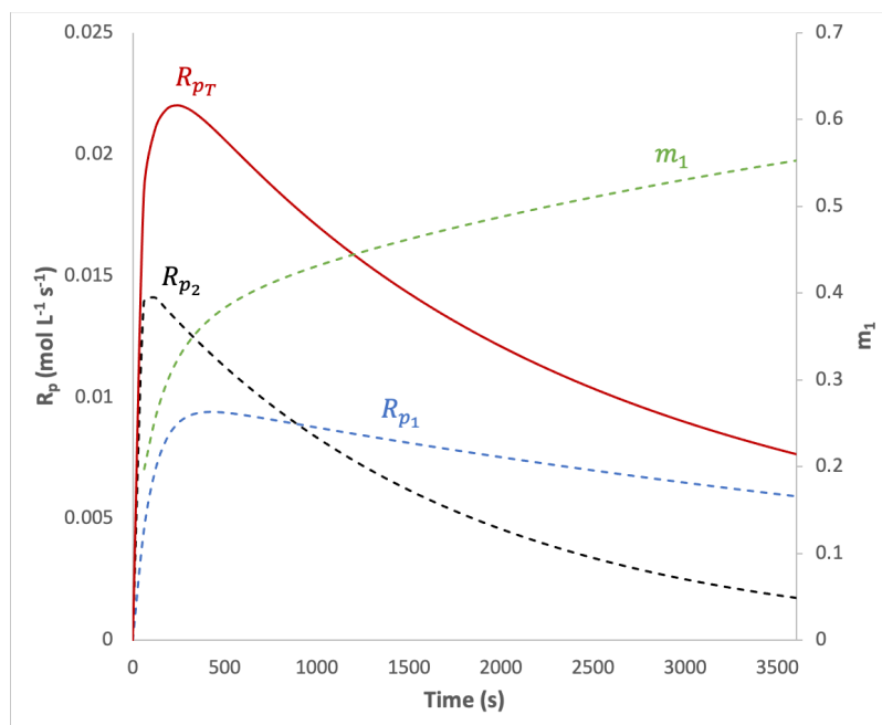
Figure 13 Polymerization rates for a dual site catalyst. Model parameters: 1) f_{p1} = 1 \times 10^5 \text{ s}^{-1} , f_{d1} = 1 \times 10^{-2} \text{ s}^{-1} , f_{a1} = 1.5 \times 10^{-4} \text{ s}^{-1} , [C_0]_1 = 1 \times 10^{-8} \text{ mol} \cdot \text{L}^{-1} , M_{n1} = 200\,000 , 2) f_{p2} = 1.5 \times 10^5 \text{ s}^{-1} , f_{d2} = 5 \times 10^{-2} \text{ s}^{-1} , f_{a2} = 6 \times 10^{-4} \text{ s}^{-1} , [C_0]_2 = 1 \times 10^{-8} \text{ mol} \cdot \text{L}^{-1} , M_{n2} = 40\,000 . V_R = 1 \text{ L} , \bar{M} = 28 (polyethylene).
