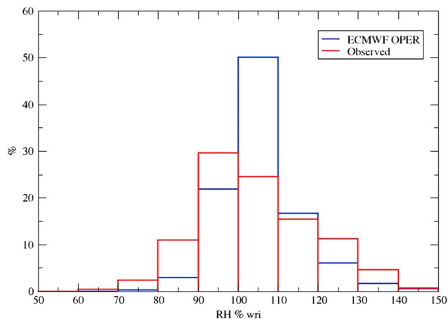
Figure 1. The observation and ECMWF operational analysis of the distribution of RH i in the surface atmosphere of Dome C, East Antarctica, in 2015. Adapted from Genthon et al. (2017). ECMWF = European Centre for Medium-Range Weather Forecasts; RH = relative humidity.
