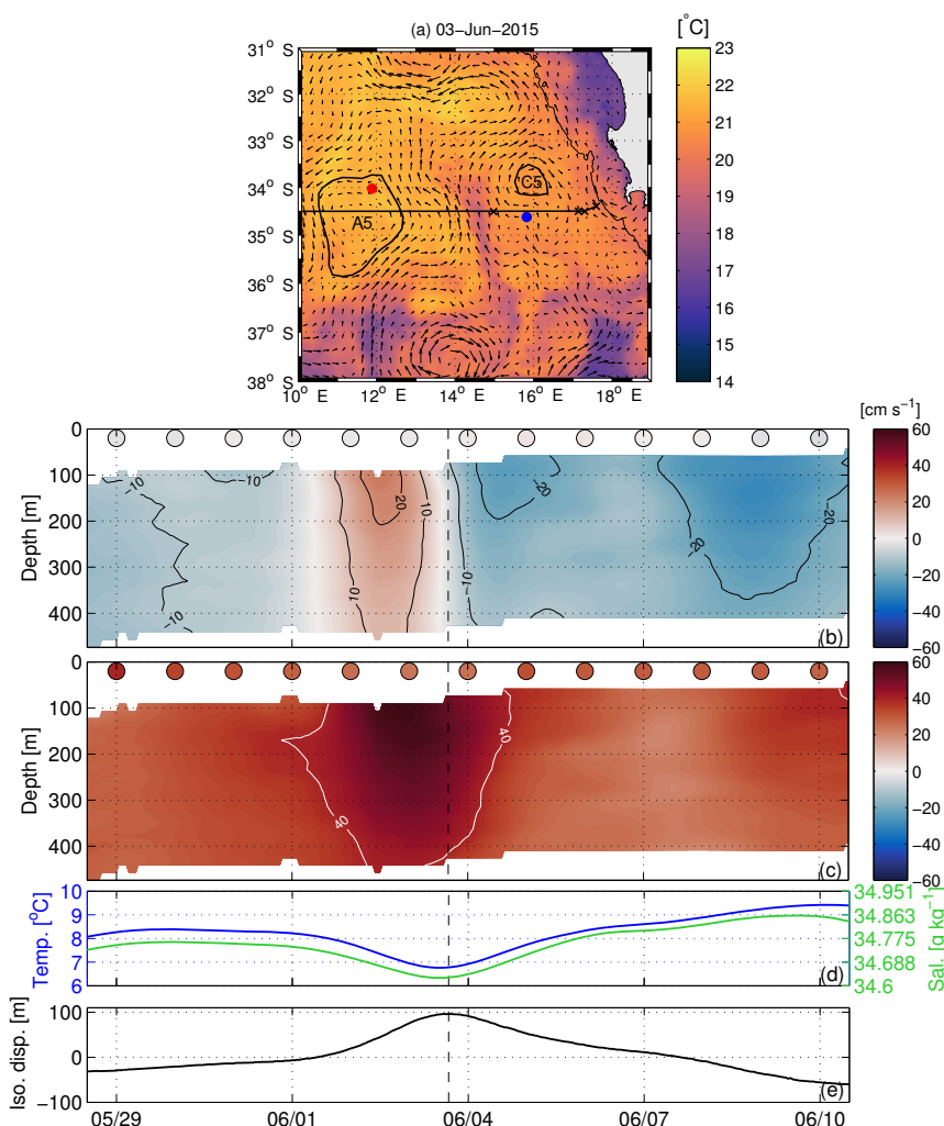
Figure 9. Cyclonic eddy: (a) SST satellite image for selected date (vertical black line on the time series). Vertical–temporal section of the u component (b) and v component (c) of the current speed measured from the upward-looking ADCP at M4. The colored circles at the top of the section show the u and v component of the current speed from altimetry data. (d) Temporal evolution of temperature (blue line) and salinity (green line) and (e) the isopycnal displacement recorded at the first SBE37 MicroCATs between 470 and 500 m depth.
