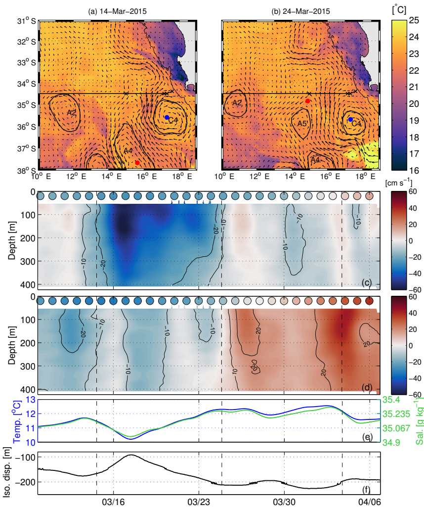
Figure 8. Anticyclonic eddy: (a, b) SST satellite images for selected dates (vertical black lines on the time series). Vertical–temporal section of the u component (c) and v component (d) of the current speed measured from the upward-looking ADCP at M4. The colored circles at the top of the section show the u and v component of the current speed from altimetry data. (e) Temporal evolution of temperature (blue line) and salinity (green line) and (f) the isopycnal displacement recorded at the first SBE37 MicroCATs between 430 and 450 m depth.
