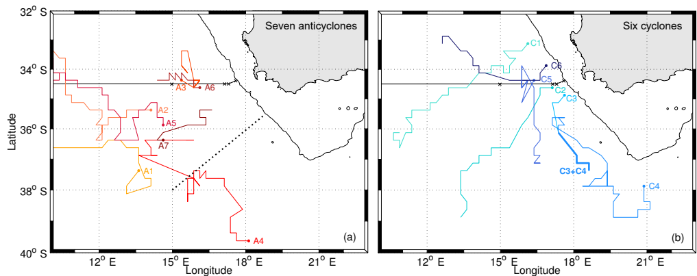
Figure 4. Eddy trajectories from 15 September 2014 to 15 December 2015 for eddies influencing the mooring measurements. The eddies are named A1–A7 (anticyclonic eddies – a ) and C1–C6 (cyclonic eddies – b ), with the numbers assigned in chronological order by the eddy-tracking scheme. The circles indicate the starting positions of an eddy track. The bold blue line in ( b ) represents the trajectory of an eddy after a merging. ( a ) The dashed black line represents the northern route of Agulhas rings defined by Dencausse et al. (2010).
