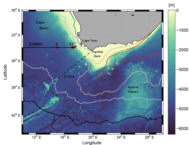
Figure 1. Study area with shaded color representing the bathymetry (m) from ETOPO1. The thin black line denotes the position of the SAMBA-east transect and the black crosses (red squares) represent the mooring (CPIES) positions with their associated numbers (1, 2, 3 and 4). The dotted black line denotes the C-line position. Annually averaged 2015 SST isotherms from the ODYSSEA data set are plotted with colored contours.
