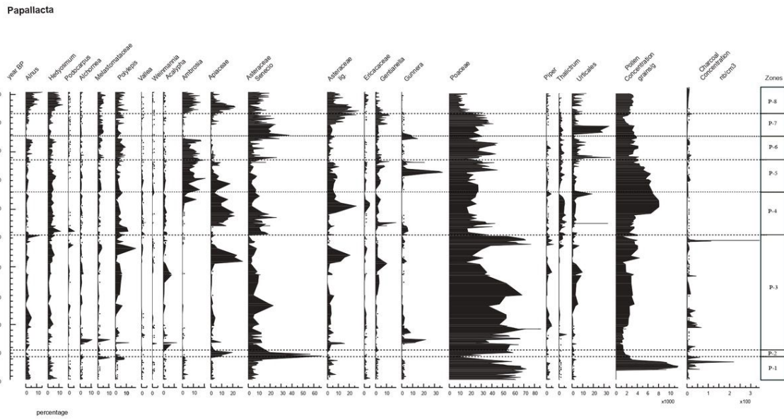
Figure 4: Percentages of 23 selected pollen and non-pollen taxa sampled from core PA1-08 plotted along an age scale. Dashed horizontal lines: statistically significant pollen assemblage zone boundaries
