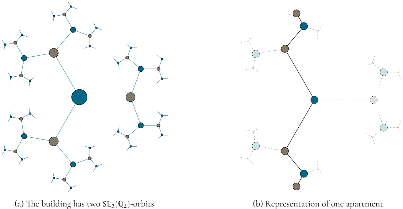
Figure 3: The building of \mathrm{PSL}_2(\mathbb{Q}_2)
